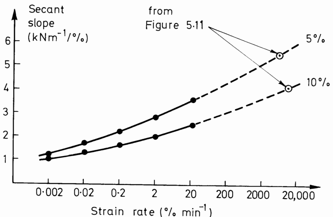
Figure 5.13 Effect of Strain Rate on Secant Slope of Figure 5.11 (at 5% and 10% strain), for Tensar SS1 (after McGown 1982)
