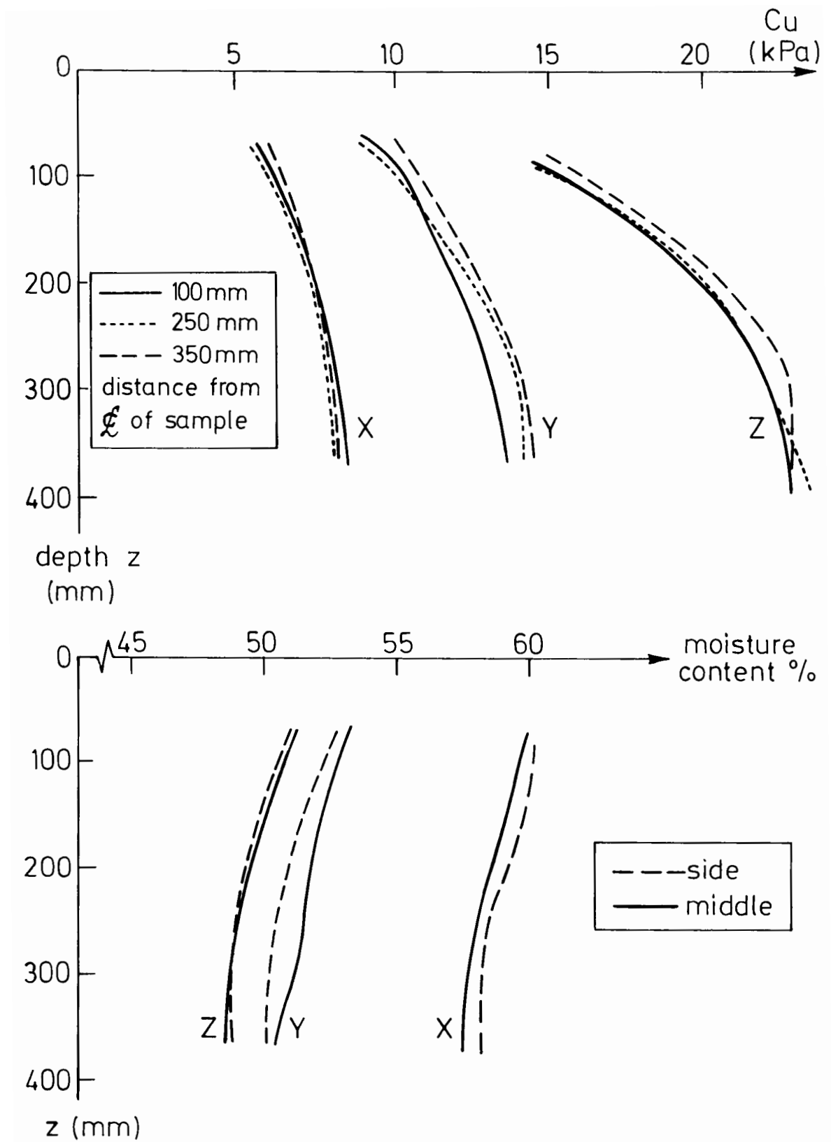
Figure 5.3 Undrained Shear Strength and Moisture content profiles with depth for Clay Samples X , Y and Z (Depth measured from original height of sample before trimming)
