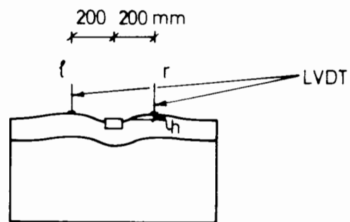
Plate 4.2 View of LVDT
