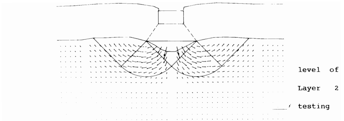
Figure 7.8 Displacement Vector plot corresponding to 50mm Footing Penetration for the reinforced test J1M (Single Increment)
