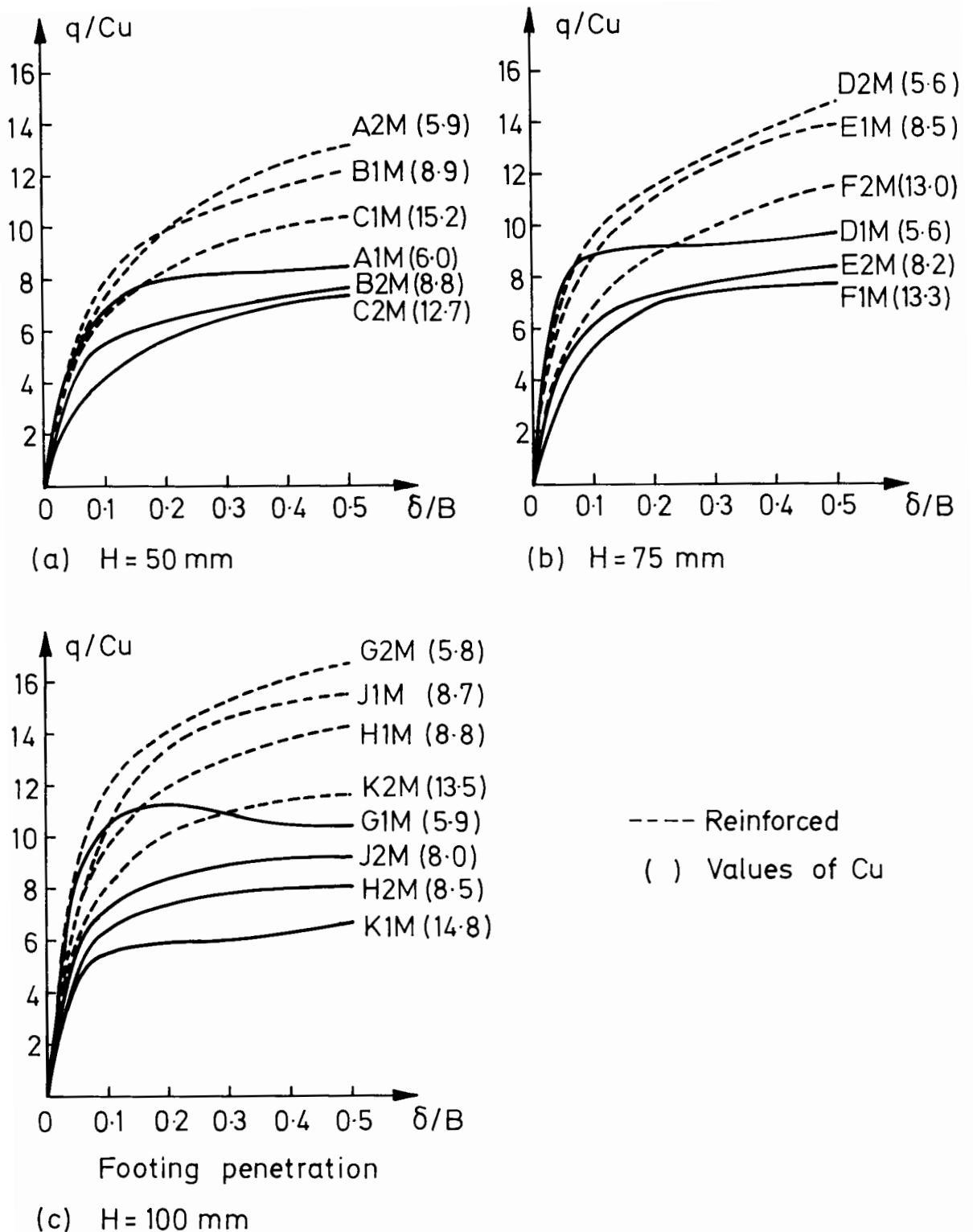
Figure 6.3 Footing Load data, normalised by C_u , plotted against normalised Footing Penetration and grouped according to Fill Thickness
