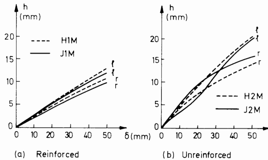
Figure 4.6 Heave versus Footing Penetration for reinforced and unreinforced tests on Samples H and J
