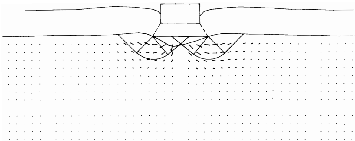
Figure 7.22 Displacement Vector plot for the unreinforced test A1M (25mm Footing Penetration)
