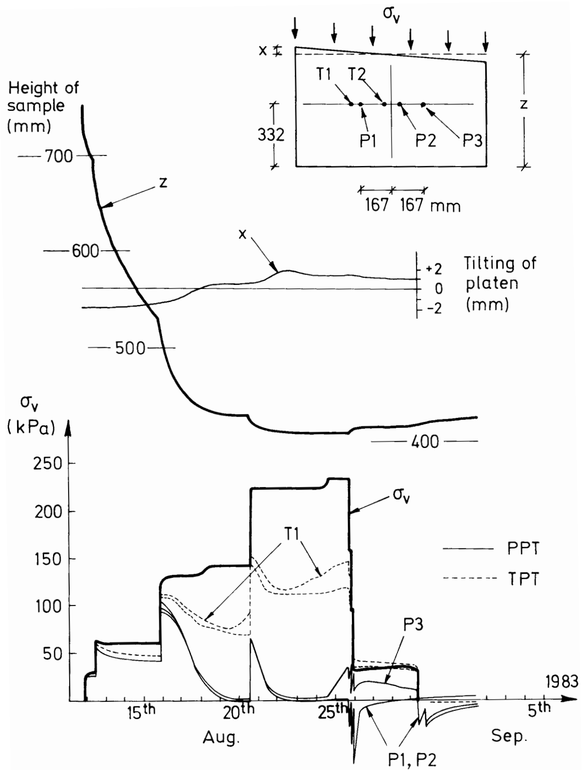
Figure 3.2 Consolidation Summary for Sample J (Nominal C_u = 9\text{kPa} )
