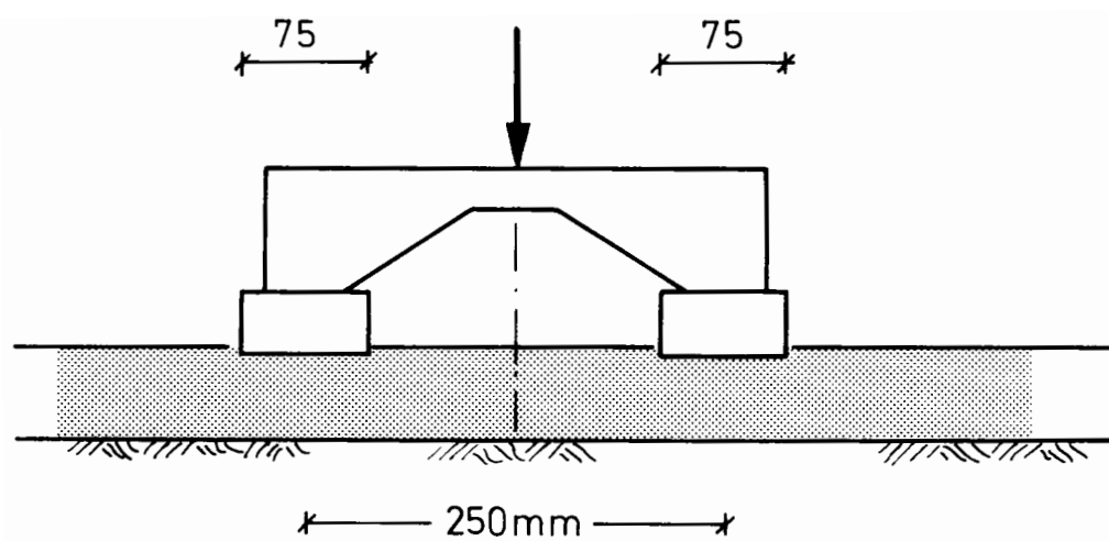
Figure 4.21 Dual Footing
