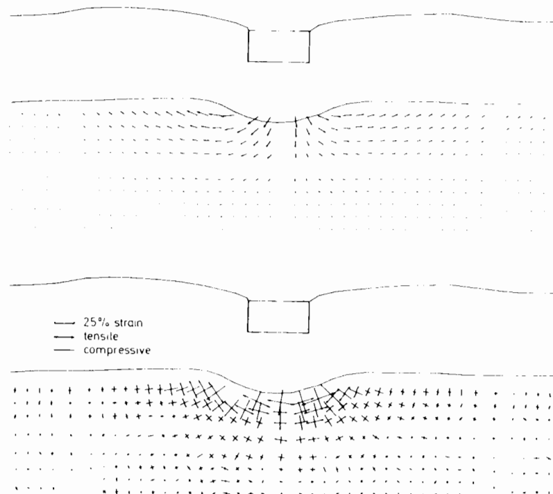
a) H1M (Reinforced test)
