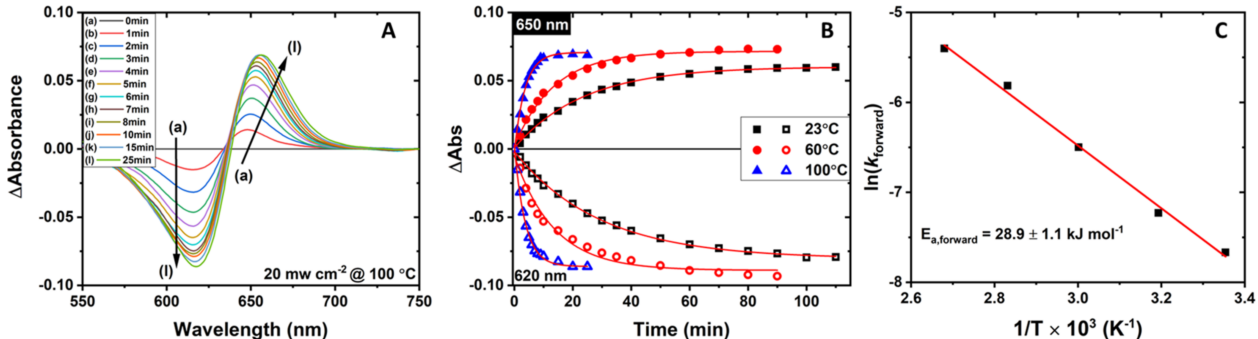
Figure 7: Work of Elmelund et al. tracking the speed of halide segregation in MAPb(Br 0.5 I 0.5 ) 3 perovskite films at different temperatures. 40 The films were illuminated with a white light source at 20 mW cm -2 ( \sim 0.2 sun) intensity. (a): Changes in the absorption spectra of an illuminated sample over time as compared to the pre-illumination measurement of absorption. The temperature of the sample was 100 °C. (b): Growth of the sub-bandgap absorption (measured at 650 nm, solid symbols) and shrinkage of the above-bandgap absorption (measured at 620 nm, open symbols) over time for perovskite samples at 23, 60, and 100 °C (black squares, red circles and blue triangles respectively). (c): Plot of the natural log of the rate constant associated with halide segregation versus the inverse temperature of the perovskite material, with the linear trend highlighting an Arrhenius relation. The rate constant associated with halide segregation was obtained from mono-exponential fits to the data in (b). Reprinted with permission from [Ref. 40]. Copyright 2019, American Chemical Society.
