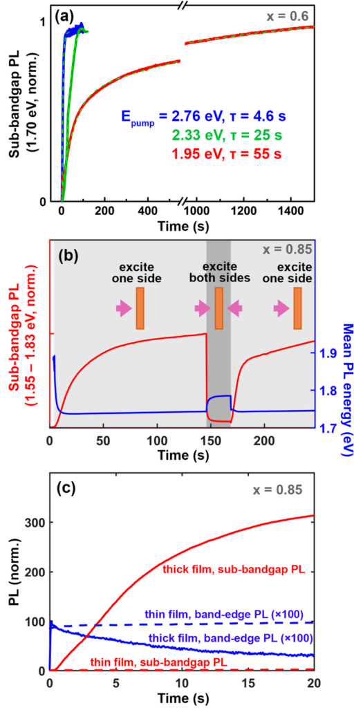
Figure 6: Data presented by Barker et al. suggesting a link between the illumination profile within a perovskite thin film and the amount of halide segregation induced in the material. 38 (a): The emergence of sub-bandgap PL from a \text{MAPb}(\text{Br}_{0.6}\text{I}_{0.4})_3 film under illumination at different photon energies ( E_{\text{pump}} ) and intensities, but similar photon flux. (b): Changes in the sub-bandgap PL (associated with iodide enriched domains) and average PL energy emitted from a \text{MAPb}(\text{Br}_{0.6}\text{I}_{0.4})_3 film under either one- or two- (one incident on each side of the film) beam illumination of 100 \text{ mW cm}^{-2} ( \sim 1 sun) intensity, 405 \text{ nm} wavelength each. (c): Changes in the PL intensities emitted from thick ( 280 \text{ nm} ) and thin ( 70 \text{ nm} ) \text{MAPb}(\text{Br}_{0.85}\text{I}_{0.15})_3 perovskite films under the same, one-sided illumination as in (b). Reprinted with permission from [Ref. 38], https://doi.org/10.1021/acsenergylett.7b00282 . Further permissions related to the material excerpted should be directed to the ACS.
