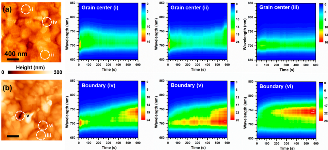
Figure 2: Work by Tang et al. highlighting how stability against halide segregation differs between the grain centres and boundaries of a \text{MAPb}(\text{Br}_{0.3}\text{I}_{0.7})_3 perovskite thin film. 97 (a) and (b): Topography of the film, with regions of interest circled as grain centres (regions i-iii) or grain boundaries (iv-vi). Plotted is the emitted PL from each region while individually illuminated under 500\,000\text{ mW cm}^{-2} ( \sim 5000 sun), 636 nm illumination for 10 minutes. Only the PL emitted from the grain boundaries shows signs that halide segregation is occurring, through the emergence of redshifted features. Reprinted with permission from [Ref. 97]. Copyright 2018, American Chemical Society.
