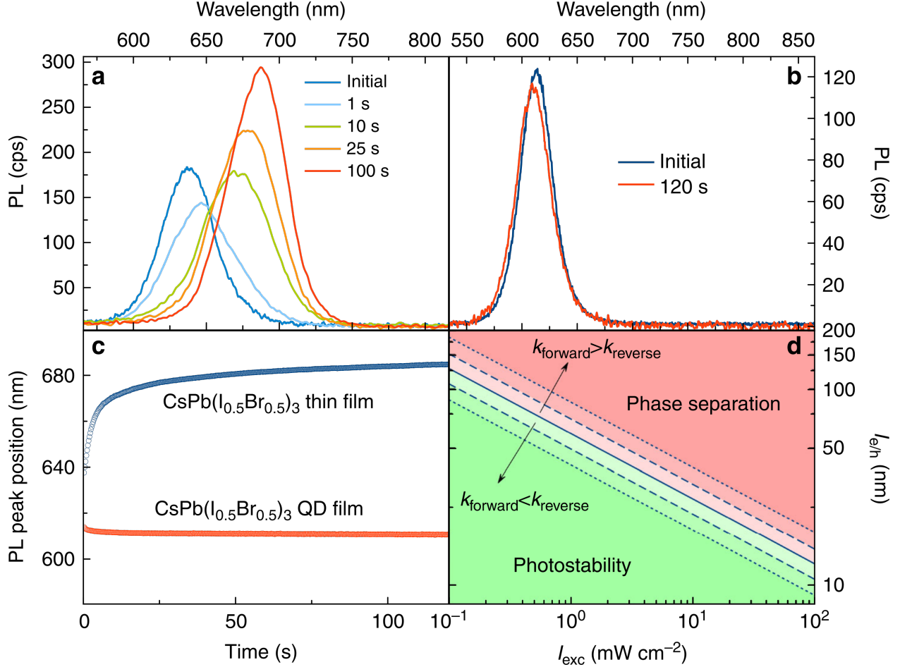
Figure 3: Data presented by Draguta et al. showing the stability of films made from perovskite nanocrystal solutions versus that for standard polycrystalline thin perovskite films. 39 (a) and (b): Evolution of the PL emitted from both a CsPb(Br 0.5 I 0.5 ) 3 perovskite thin film (a) and a nanocrystal film (b) under 60 mW cm -2 ( \sim 0.6 sun), 405 nm illumination. (c): The tracked PL peak position from (a) and (b), highlighting that only the bulk thin film experienced a PL redshift and halide segregation. (d): Theoretically predicted phase diagram of the photostability of MAPb(Br x I (1-x) ) 3 perovskites as a function of illumination intensity ( I_{exc} ) and excited charge-carrier diffusion length ( l_{e/h} ). Reprinted from [Ref. 39]. Copyright 2017, Nature Publishing Group.
