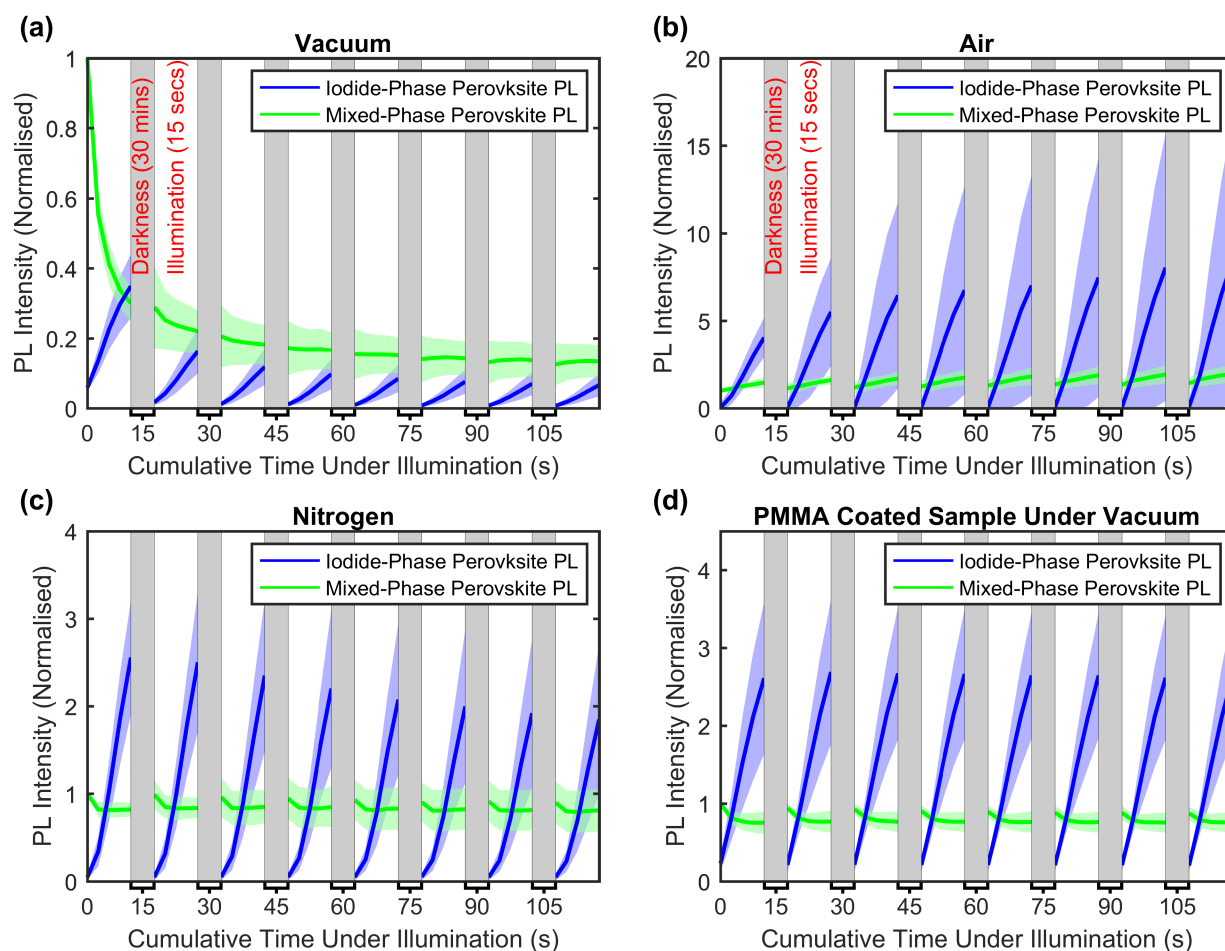
Figure 5: Atmospheric dependence of spectral shifts resulting from light-induced halide segregation in \text{MAPb}(\text{Br}_{0.5}\text{I}_{0.5})_3 . 103 Films were subjected to 8 periods of 15 s-long illumination at 60 \text{ mW cm}^{-2} ( \sim 0.6 sun) intensity and 400 nm wavelength under different atmospheric conditions. All consecutive illumination periods were separated by 30 minutes in darkness (indicated by the grey zones). The solid blue lines indicate the average intensity of the emitted below-bandgap PL (integrated from 720-770 nm) attributed to iodide-rich phases, and the solid green lines indicate the average intensity of the initial mixed-phase perovskite PL (integrated from 640-690 nm). The averages were taken over several experimental runs on fresh sections of perovskite. The shaded blue and green regions indicate the values within one standard deviation of their respective averages. (a): Perovskite films held under vacuum ( \sim 0.2 mbar). (b): Films held under ambient air. (c): Films held under pressurised nitrogen ( \sim 2 bar). (d): Films topped with a layer of PMMA and held under vacuum ( \sim 0.2 mbar) Reprinted with permission from [Ref. 103], https://doi.org/10.1021/acseenergylett.8b02002 . Further permissions related to the material excerpted should be directed to the ACS.
