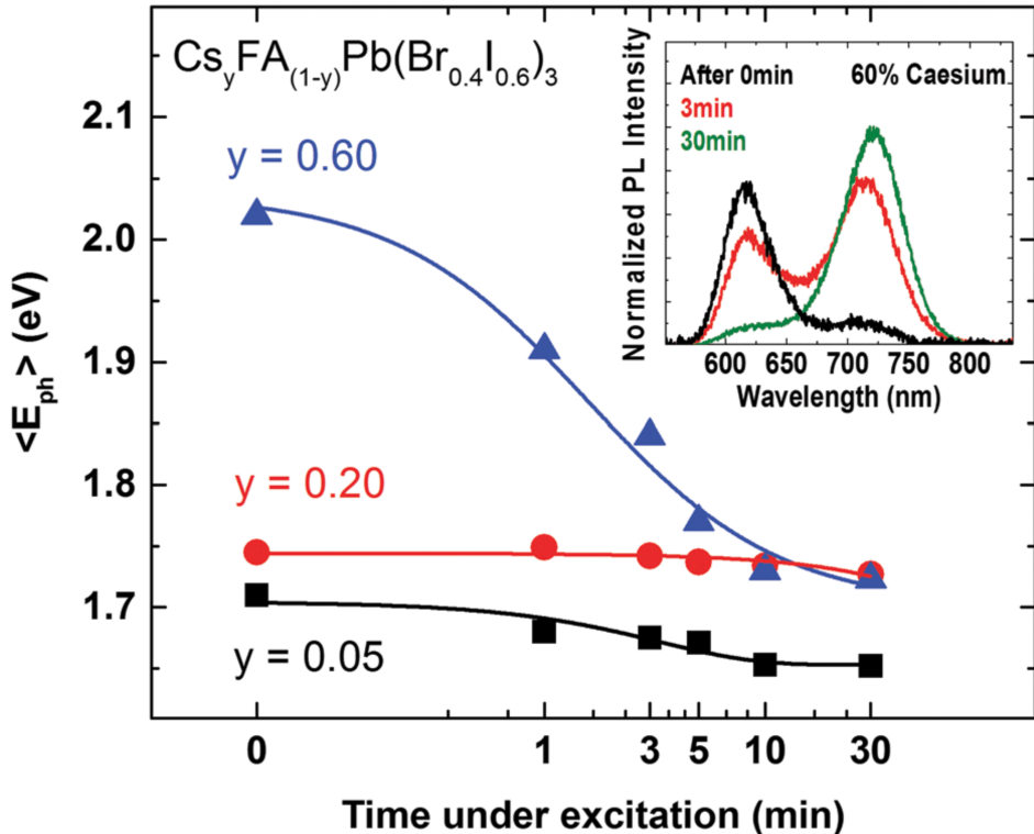
Figure 1: Work by Rehman et al. highlighting how changes of the FA/Cs ratio on the A-cation sites of a lead halide perovskite affects the rate of halide segregation under illumination. 9 The main figure plots the average PL photon energy \langle E_{\text{ph}} \rangle over time for \text{Cs}_y\text{FA}_{(1-y)}\text{Pb}(\text{Br}_{0.4}\text{I}_{0.6})_3 perovskite films with y=0.05 , y=0.2 , and y=0.6 under 100 \text{ mW cm}^{-2} ( \sim 1 sun), 400 \text{ nm} illumination. For 20% Cs little energetic shift is observed, suggesting negligible halide segregation. The inset shows the spectral evolution of the PL emitted by the y=0.6 sample. [Ref. 9] – Published by The Royal Society of Chemistry.
