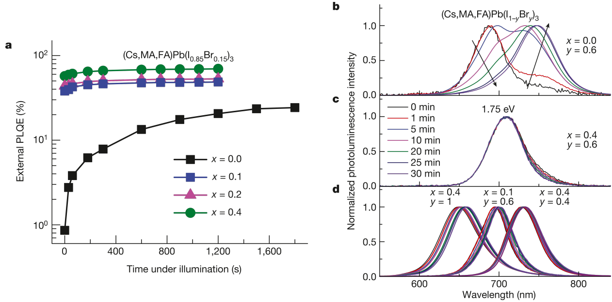
Figure 4: Data presented by Abdi-Jalebi et al. highlighting the effects of a potassium iodide passivating agent on the photostability of (\text{Cs}_{0.06}\text{MA}_{0.15}\text{FA}_{0.79})\text{Pb}(\text{Br}_y\text{I}_{(1-y)})_3 perovskite films. 73 (a): External PL quantum efficiency over time under illumination ( 60 \text{ mW cm}^{-2} , \sim 0.6 sun, 532 \text{ nm} ) for 4 perovskite films with different ratios of potassium iodide to A-site cations ( x ) added to the perovskite precursor solutions. The external PL quantum efficiency increases in perovskite films undergoing halide segregation due to the funnelling and concentration of excited charge carriers in the forming regions of low-bandgap perovskite. (b): PL spectra observed over 30 minutes for a (\text{Cs}_{0.06}\text{MA}_{0.15}\text{FA}_{0.79})\text{Pb}(\text{Br}_{0.6}\text{I}_{0.4})_3 film with no passivating agent ( x=0 ) under the same illumination conditions as in (a). (c) and (d): PL spectra over 30 minutes for perovskite films with varying halide content ( y=0.6 (c), y=1, 0.6, 0.4 (d)) and varying amounts of passivating agent added ( x=0.4 (c), x=0.4, 0.1, 0.4 (d)) under the same illumination conditions as in (a). Reprinted by permission from Springer Nature: Nature [Ref. 73], 2018.
