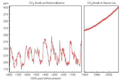
Figure 4: Levels of atmospheric \text{CO}_2 .
