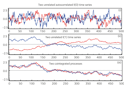
Figure 8: Pairs of artificial time series: (i) unrelated I(0) ; (ii) unrelated I(1) ; (iii) cointegrated.
