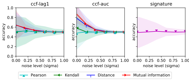
Figure 4: Average and confidence interval for accuracy by lead-lag detection method in the cosine setting.
