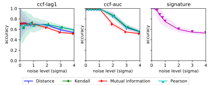
Figure 3: Average and confidence interval for accuracy by lead-lag detection method in the linear setting.
