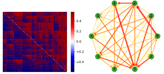
Figure 1: Left: Heatmap of the double-sorted lead-lag matrix A - A^T ; positive entries in the matrix correspond to a leading relationship between the stock depicted on the vertical axis with respect to the stock depicted on the horizontal axis. Right: Meta-flow network for Hermitian RW clusters; clusters are represented by nodes and larger edge weights are depicted by bolder lines.
