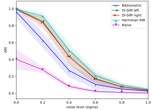
Figure 6: Average and confidence interval for the ARI by clustering method in the cosine setting.
