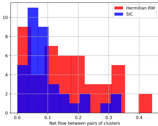
Figure 7: Histogram of Hermitian RW and SIC clustering meta-flow network edge weights. We see that the edge weights for the meta-flow network corresponding to a Hermitian RW clustering tend to be larger than the edge weights for the meta-flow network corresponding to a SIC clustering.
