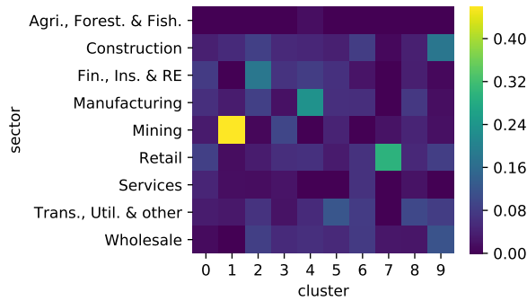
Figure 2: The Jaccard similarity coefficient between Hermitian RW and industry clusters (SIC)
