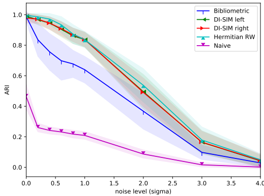
Figure 5: Average and confidence interval for the ARI by clustering method in the linear setting.
