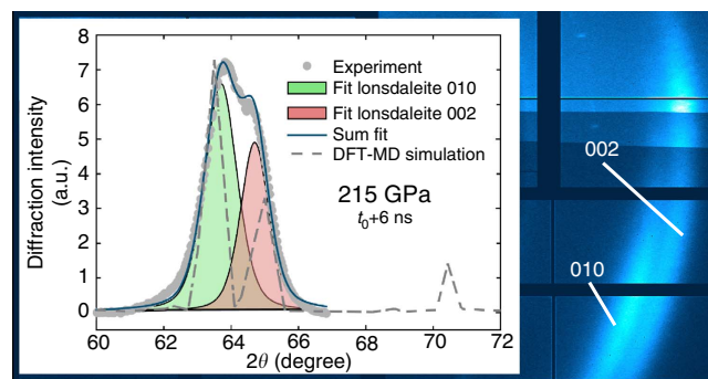
Figure 3 | Diffraction from lonsdaleite. When compressing pyrolytic graphite to pressures above 170 GPa, we observe two strong diffraction peaks consistent with lonsdaleite (010) and (002) planes. The grey-dashed line shows a DFT-MD simulation of the lonsdaleite phase at 4.4 \text{ g cm}^{-3} and 6,000 K, resulting in a pressure of 205 GPa, which is in qualitative agreement with the observed diffraction pattern. As the range of detectable diffraction angles ends at 2\theta = 68 degrees in our experiments, the (011) peak at 2\theta = 70.5 degrees is not recorded. The occurrence of partial diffraction rings shows a preferred orientation of the crystallites that is compatible with the preferred orientation of the initial pyrolytic graphite sample.
