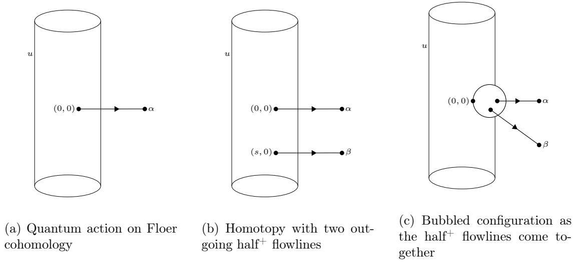
Figure 3.5: To show the quantum action on Floer cohomology (A) satisfies \alpha * (\beta * \tilde{x}) = (\alpha * \beta) * \tilde{x} , construct a homotopy with two half + flowlines as in (B). The limit s \rightarrow \infty gives the left-hand side \alpha * (\beta * \tilde{x}) as the Floer solution breaks, while the limit s \rightarrow 0^+ gives the bubbled configuration (C) which is homotopic to the right-hand side (\alpha * \beta) * \tilde{x} .
