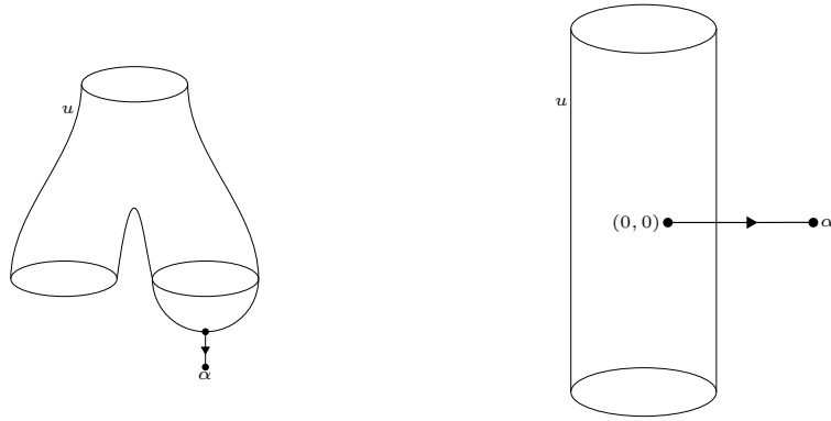
(a) Pair-of-pants product with PSS map
