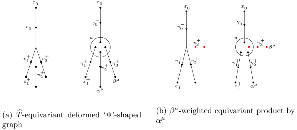
Figure 3.2: The \widehat{T} -equivariant deformed ‘ \Psi ’-shaped graphs that \Psi counts are the same configurations that the \beta^\mu -weighted equivariant product by \alpha^\mu counts. Only the interpretation of the flowline [v_3^+, \gamma_3^+] changes between the two maps.
