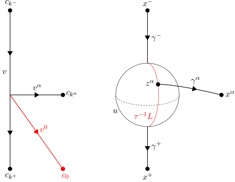
Figure 2.5: The map K_\alpha counts equivalence classes of tuples like the weighted equivariant quantum Seidel map in Figure 2.4, however with an additional flowline v^0 in S^\infty . Moreover, we restrict to tuples which satisfy z^\alpha \in \tau^{-1}L , where \tau = \tau_0(v^0(\infty)) is determined by the additional flowline in S^\infty .
