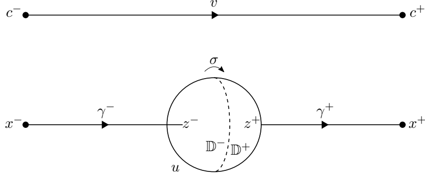
Figure 2.3: The equivariant quantum Seidel map counts equivalence classes of quadruples (v, \gamma^-, \gamma^+, u) . The map u is a section of the clutching bundle which twists the fibres by \sigma when passing from the upper hemisphere \mathbb{D}^- to the lower hemisphere \mathbb{D}^+ . The flowlines \gamma^\pm map to the manifold M , which is identified with the fibres of the clutching bundle over the poles z^\pm .
