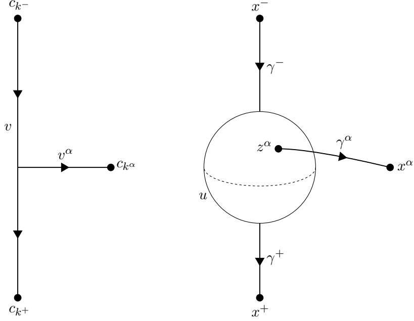
Figure 2.4: The weighted equivariant quantum Seidel map counts equivalence classes of septuples (v, \gamma^+, \gamma^-, u; v^\alpha, \gamma^\alpha, z^\alpha) . The section u of the clutching bundle intersects the flowline \gamma^\alpha over the point z^\alpha \in S^2 .
