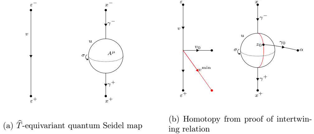
Figure 3.3: An additional flowline v^{\min} in E\hat{T} is used to describe a path between the poles. It is from this path that the half + flowline \gamma_0 flows.
