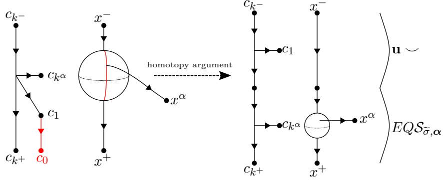
Figure 2.6: When the flowline v^0 breaks, we can use a homotopy argument to split the moduli space into multiplication by \mathbf{u} and the weighted equivariant Seidel map. The flowline from c_1 to c_0 contains redundant information so we omit it.
