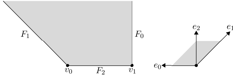
Figure 3.12: The moment polytope and the inner normal fan for \mathcal{O}_{\mathbb{P}^1}(-1) .
