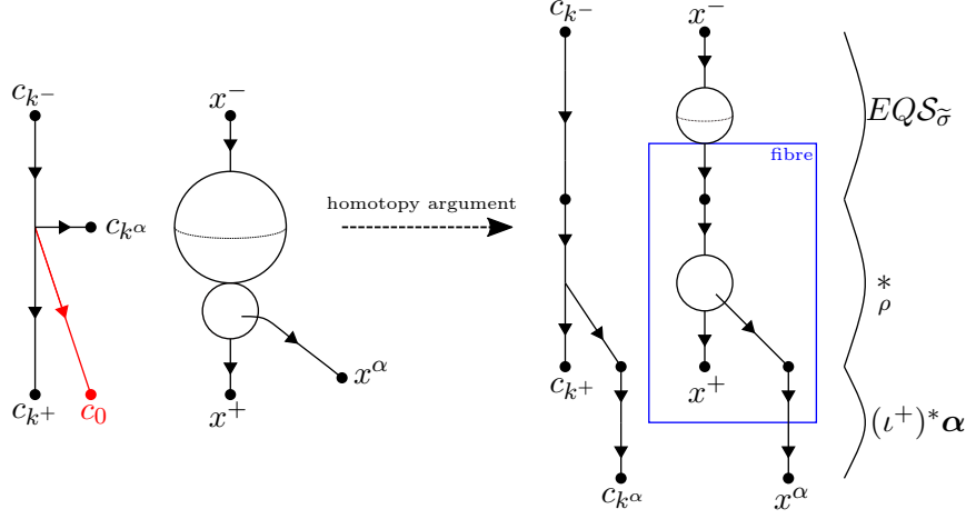
Figure 2.7: When the section bubbles over the south pole, we can use a homotopy argument to get an equivariant quantum product in the fibre above the south pole followed by the map EQS_{\tilde{\sigma}} . The flowline to c_0 is redundant, so we remove it.
