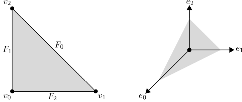
Figure 3.10: The moment polytope and the inner normal fan for \mathbb{P}^2 .
