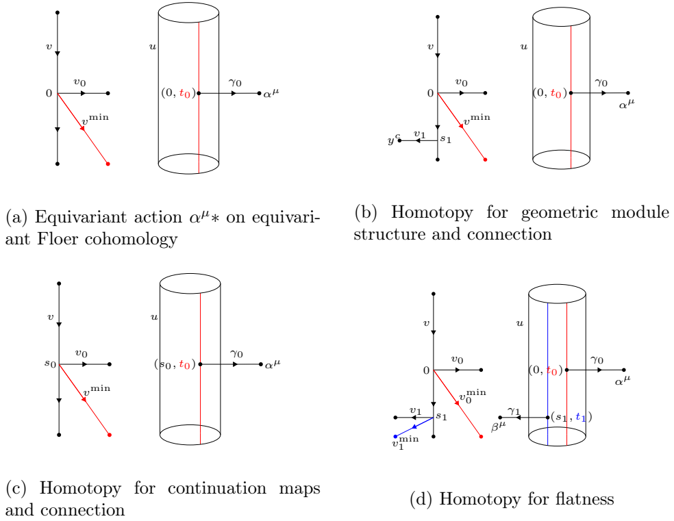
Figure 3.6: The connection comprises a formal differentiation operation and the equivariant action \alpha^\mu* in (A). The action is modified into three different homotopies which are used to show the connection is compatible with the geometric H^*(B\hat{T}) -module structure (B), compatible with continuation maps (C) and flat (D).
