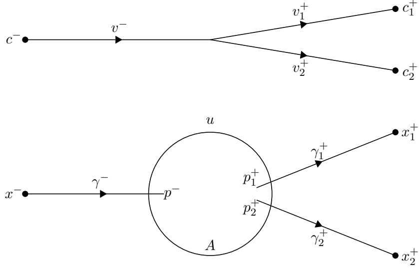
Figure 2.2: The equivariant quantum product counts equivalence classes of septuples (v^-, v_1^+, v_2^+, \gamma^-, \gamma_1^+, \gamma_2^+, u) . The ‘Y’-shaped graph above maps to S^\infty while the configuration below the graph maps to M .
