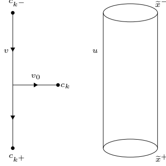
Figure 2.1: The geometric module action uses a Morse ‘Y’-shaped flowline on S^\infty .
