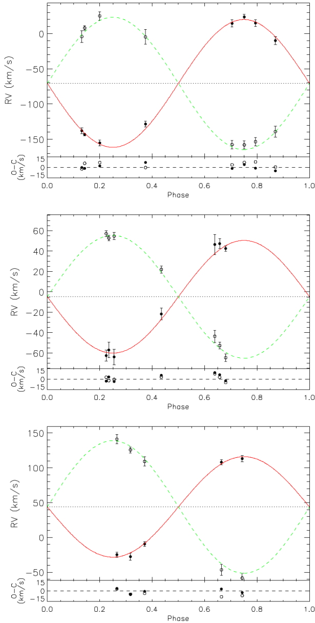
Figure 8. Primary and secondary RV curves for the MEBs. Top: 19b-2-01387 ; Middle: 19c-3-01405 ; Bottom: 19e-3-08413 . The solid black circles are RV measurements for the primary star, while open circles denote the secondary star RV measurements. The solid red lines are the model fits to the primary RVs and the dashed green lines are the fits to the secondary RVs, fixed to the systemic velocity of their respective primaries. The horizontal dotted lines mark the systemic velocities. The error bars are from IRAF.FXCOR but are scaled so that the reduced \chi^2 of the model fit is unity. They are merely an indication of the signal-to-noise of the individual spectra and the mismatch between the template and data. Under each RV plot is a panel showing the residuals of the best-fits to the primary and secondary RVs. Note the change in scale for the y-axis. The typical RV error for each component is given in Table 10 by the RMS of their respective residuals.
