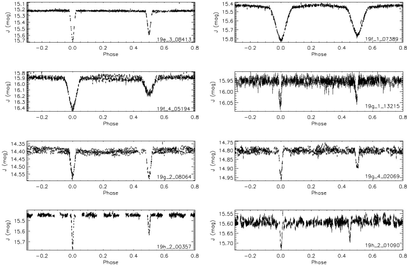
Figure A2. cont... Phase-folded light curves of the MEBs discovered in the WTS 19hr field with J \leq 16 mag.
