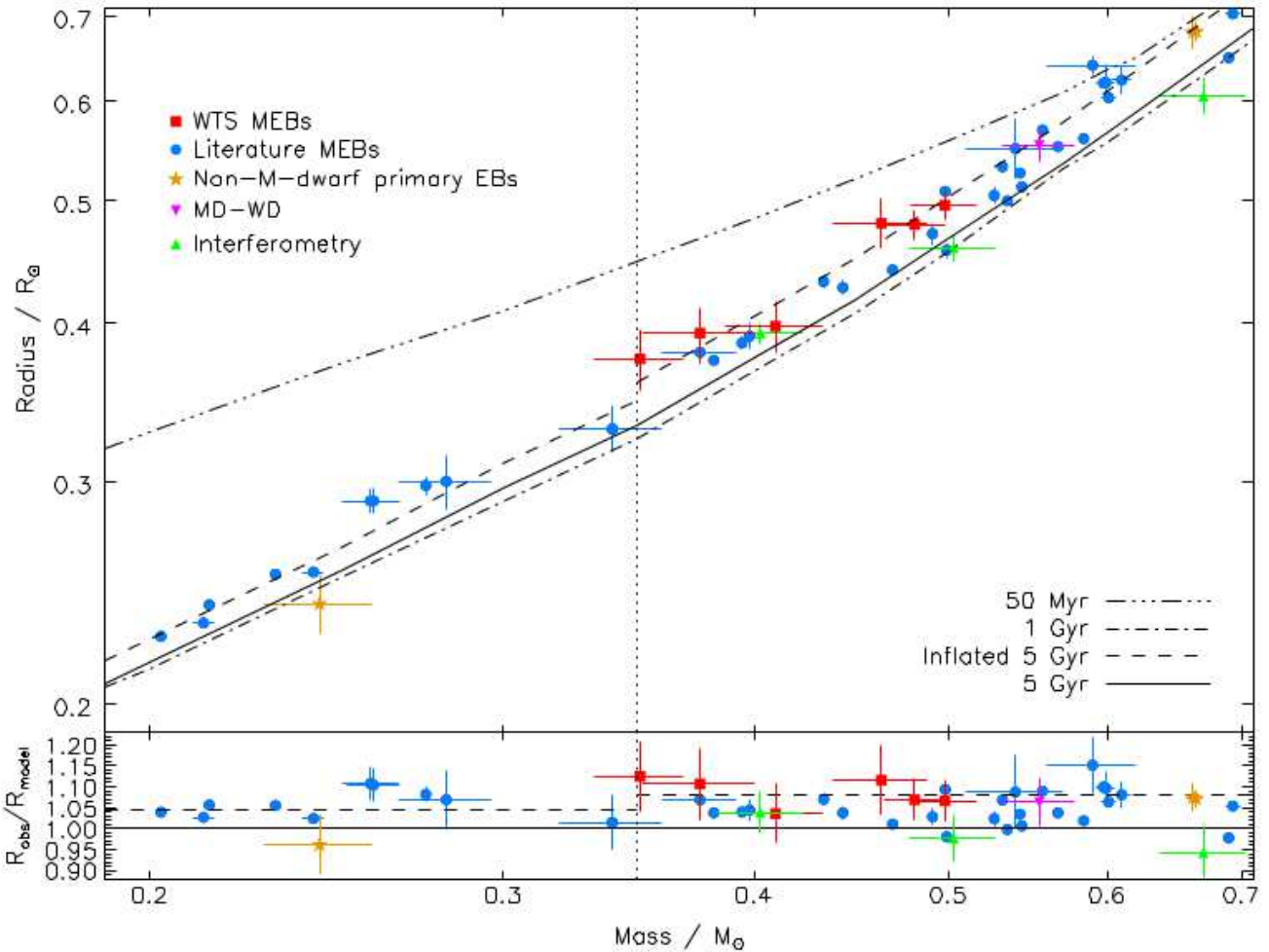
Figure 10. The mass-radius diagram for low-mass stars. The filled circles show literature MEB values with reported mass errors < 6\% and radius errors < 6.5\% . Also shown are literature values for i) the low-mass secondaries of eclipsing binaries with primary masses > 0.6M_{\odot} , ii) M-dwarfs found in M-dwarf - white dwarf eclipsing binaries (MD-WD), and iii) radius measurements of single M-dwarfs from interferometric data. The red squares mark the new WTS MEBs. The diagonal lines show model isochrones from the Baraffe et al. (1998) models ( [m/H] = 0 , Y = 0.275 and L_{\text{mix}} = H_P ), while the vertical dotted line marks the onset of fully-convective envelopes (Chabrier & Baraffe 1997). The dashed line shows the 5 Gyr isochrone plus the average radius excess found by Knigge et al. (2011), assuming a discontinuity at the fully-convective transition. Above 0.35M_{\odot} , the model is inflated by 7.9%, but below it is only inflated by 4.5%. The bottom panel shows the radius anomaly, R_{\text{obs}}/R_{\text{model}} computed using the 5 Gyr isochrone and again the dashed line shows the corresponding average radius excess found by Knigge et al. (2011). The literature data used in these plots are given in Table A3.
