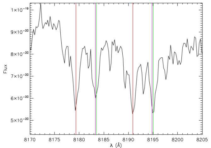
Figure 7. 19b-2-01387: A high signal-to-noise intermediate resolution spectrum taken near quadrature phase of 19b-2-01387 in the Na II doublet wavelength region which we used to measure equivalent widths to estimate the light ratio. The purple vertical lines show the rest frame wavelength of the doublet at 8183.27\text{\AA} , 8194.81\text{\AA} . The red lines mark the doublet for primary object and the green lines mark the secondary doublet lines, based on the RVs derived in Section 7.
