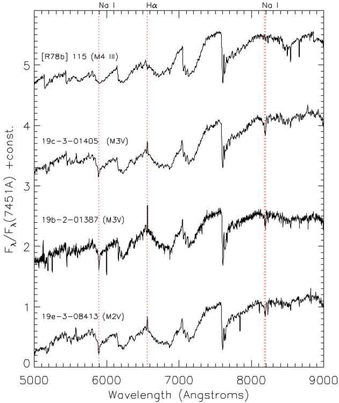
Figure 3. Low-resolution spectra of our three new MEBs plus a known M-giant star (top spectrum) for comparison. The TiO absorption band at 7100Å signifies the onset of the M-dwarf spectral types. The dotted vertical lines, from left the right, mark the Na I, H \alpha and the Na I doublet rest wavelengths in air. The Na I doublet is strong in dwarfs while the Calcium infrared triplet at 8498, 8542 and 8662Å is strongest in giants. The deep features at 7594 and 7685Å are telluric O 2 absorption. H \alpha emission is clearly present in all three MEBs.
