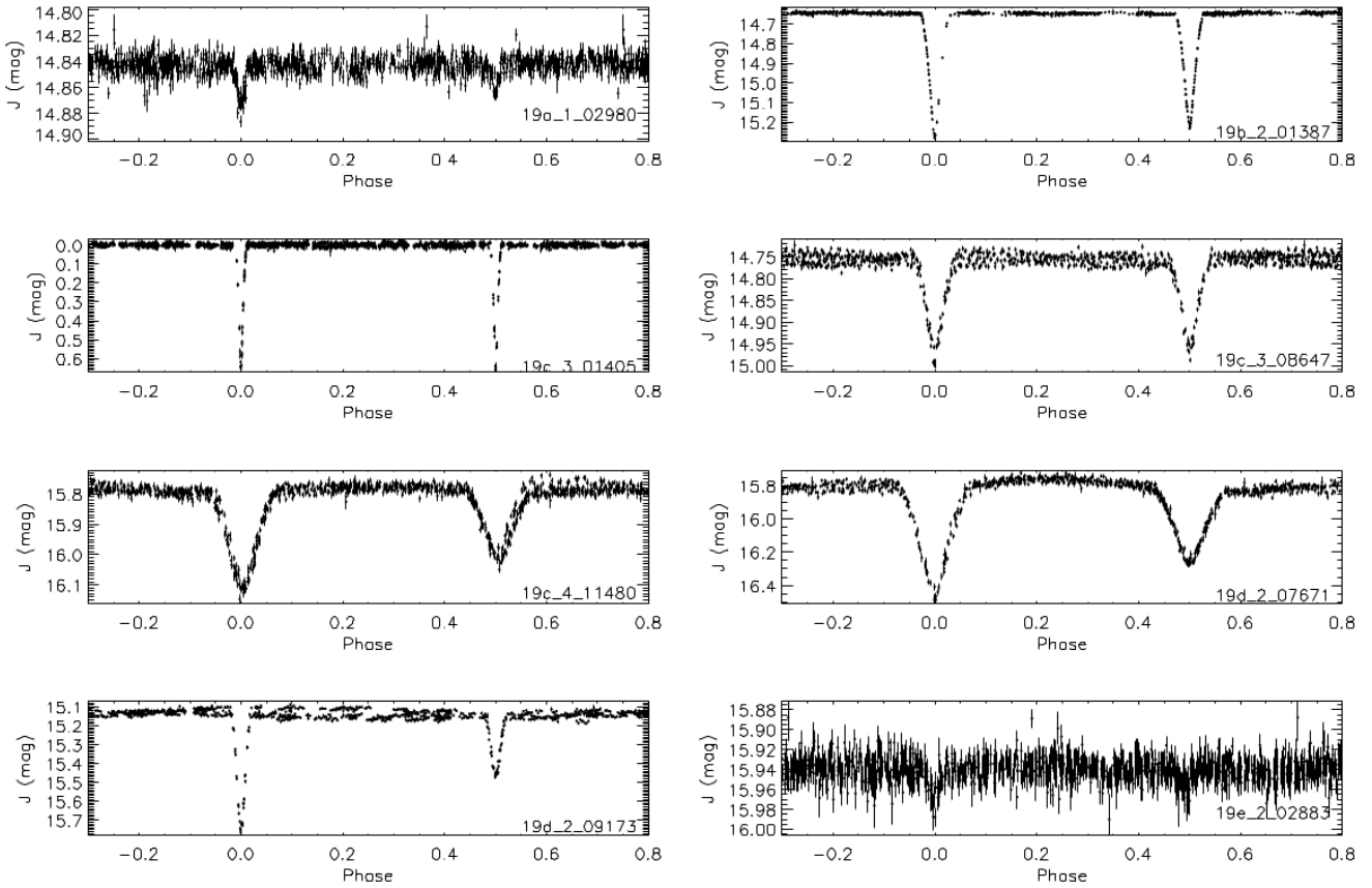
Figure A1. Phase-folded light curves of the MEBs discovered in the WTS 19hr field with J \leq 16 mag...
