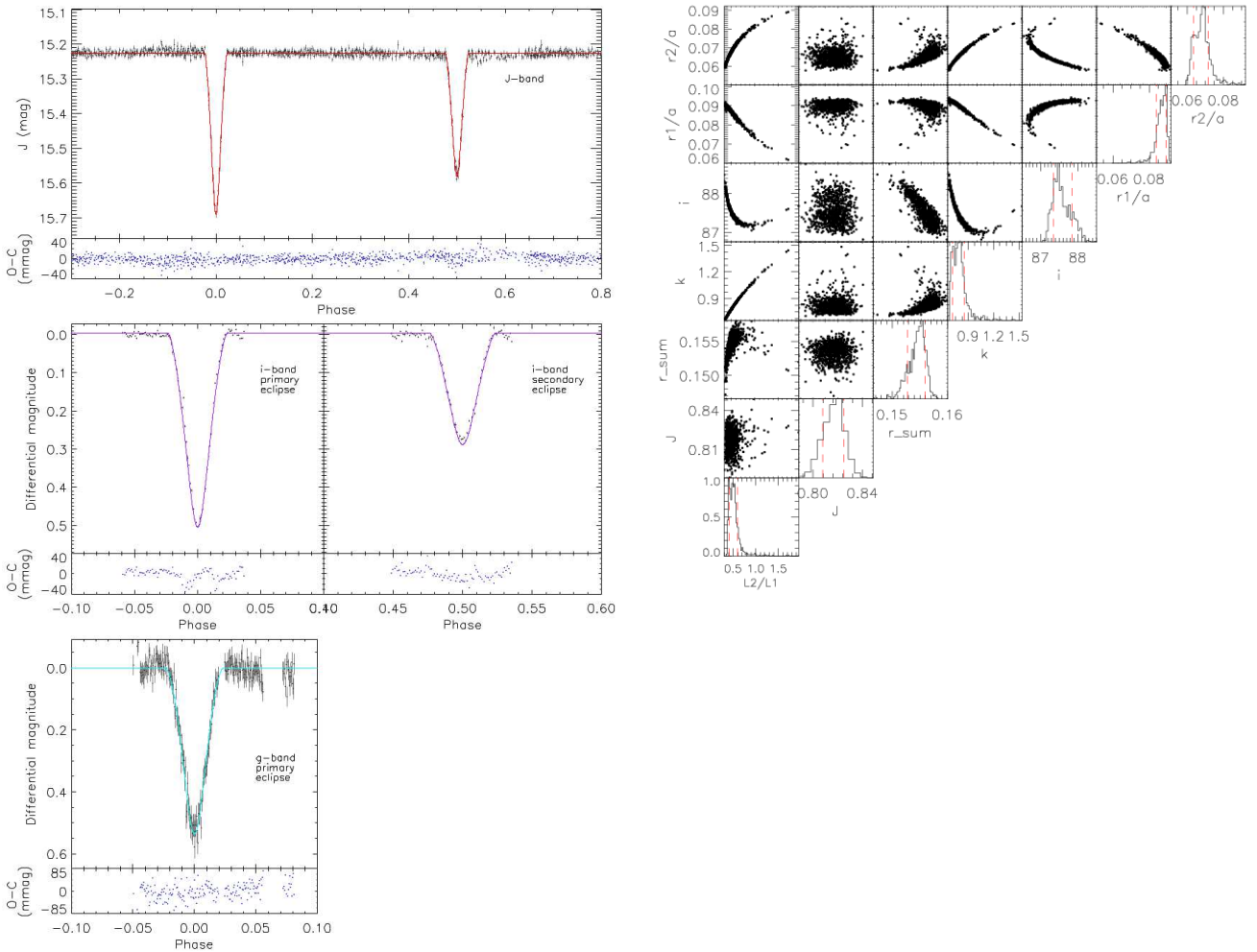
Figure 6. 19e-3-08413 Left top panel: full phase WFCAM J -band light curve. Left middle panel: INT/WFC i -band light curves of a primary and a secondary eclipse. Left bottom panel: IAC80 g -band light curve of a primary eclipse. The solid red, purple, and cyan lines show the best-fit from JKTEBOP. Right: Parameter correlations from residual permutations, which gave the larger errors on the model parameters than the Monte Carlo simulations, indicating time-correlated systematics. There are strong correlations between the light ratio, radius ratio and inclination.
