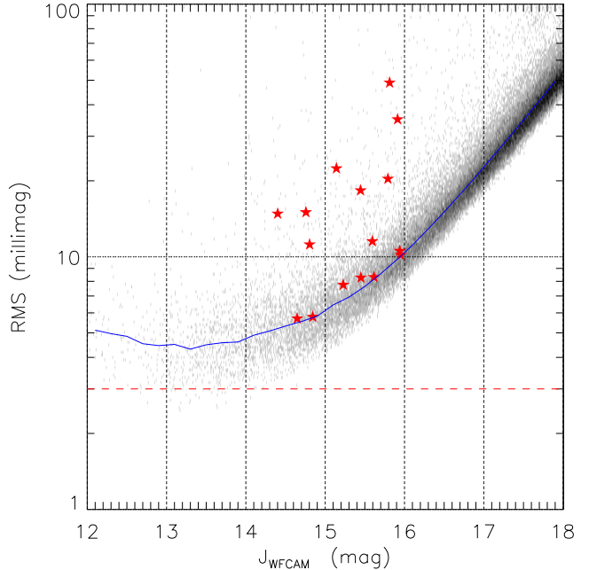
Figure 1. The RMS scatter per data point of the WTS light curves as a function of WFCAM J magnitude, for sources in the 19hr field with stellar morphological classification. The RMS is a robust estimator calculated as 1.48 \times the median of the absolute deviations. We achieve a per data point photometric precision of 3 - 5 mmag for the brightest objects, with a median RMS of \sim 1\% for J = 16 mag. Saturation occurs between \sim 12 - 13 mag as it varies across the field and with seeing. The dashed red horizontal line at 3 mmag marks the limit of our photometric precision. The blue solid curve shows the median RMS in bins of 0.2 mag. The red stars show the positions of the 16 WTS 19hr field MEBs. The shorter period MEBs sit higher in the plot. RMS values are given in Table A1
