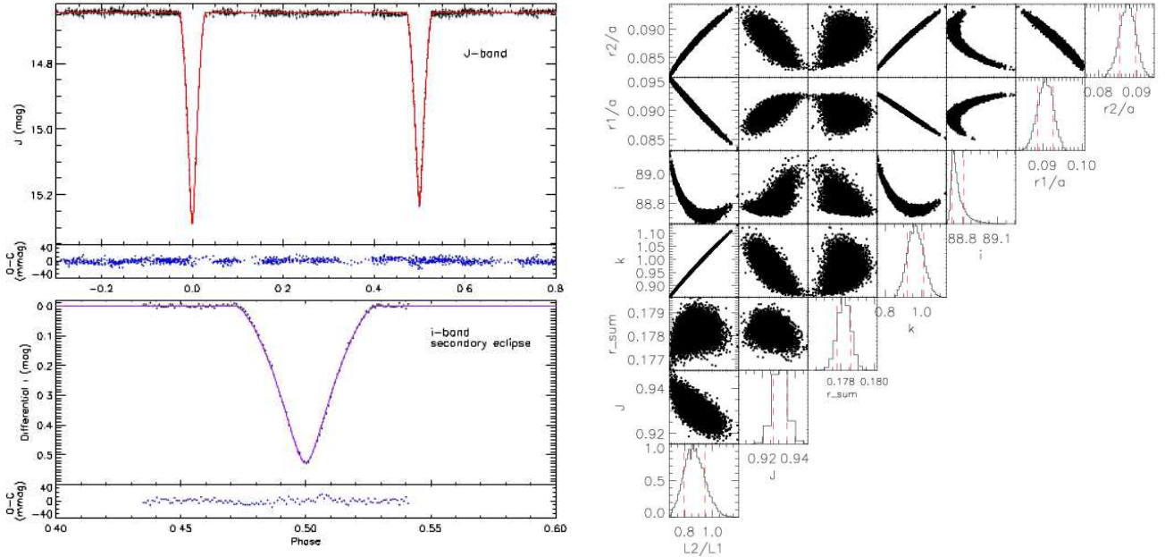
Figure 4. 19b-2-01387 Left top panel: full phase WFCAM J -band light curve. Left bottom panel: the INT/WFC i -band light curve at secondary eclipse. The solid red and purple lines show the best-fit from JKTEBOP. The blue data points in the smaller panels show the residuals after subtracting the model. Right: Parameter correlations from Monte Carlo simulations and histograms of individual parameter distributions. The red dashed vertical lines mark the 68.3% confidence interval. There is a strong correlation between the light ratio, the radius ratio, and the inclination (which is skewed), indicating the difficulty in constraining the model even with our high quality light curves.
