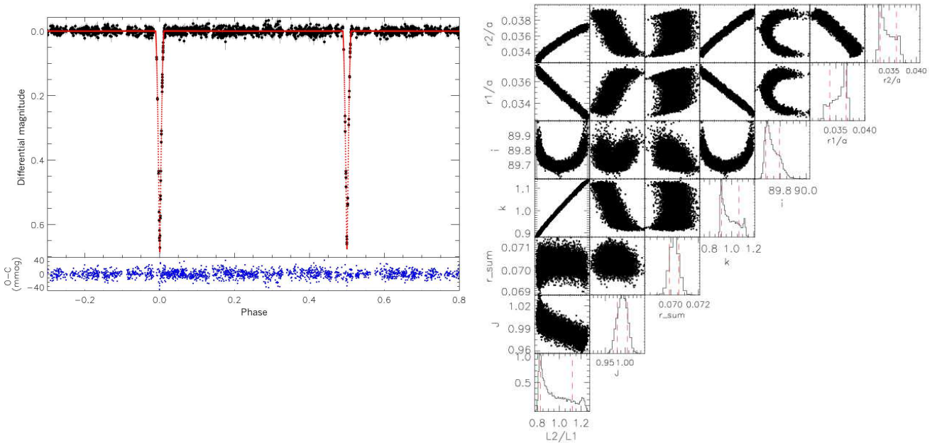
Figure 5. 19c-3-01405 Left: WFCAM J -band light curve. Lines and panels as in Figure 4. The magnitude scale is differential as we have combined light curves from two different WFCAM chips. Right: Monte Carlo results with lines as in Figure 4. Our inability to constrain the model with follow-up data results in strong correlation between the radius ratio and light ratio and parameter distributions that are significantly skewed. There are also degeneracies in the inclination which is expected given the near identical eclipse depths.
