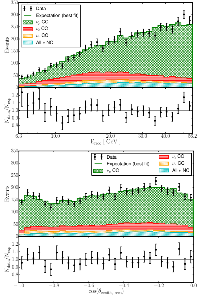
FIG. 8. Event rates shown as a function of (top) E_{reco} and (bottom) \cos\theta_{z, reco} . The various different neutrino components from Monte Carlo simulation used in the fit are shown as stacked histograms. The total expected event rate is in good agreement with the observed data, shown as black points.
