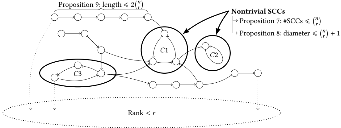
Figure 1. Graphical representation of \mathcal{K}(A) , vertex and edge labels omitted for clarity. Note that the graph can have infinitely many vertices. Propositions 7 and 8 respectively show that there are only finitely many nontrivial SCCs and they have finite diameter. Proposition 9 shows that paths avoiding nontrivial SCCs must be short. All paths in \mathcal{K}(A) are labelled by rank r matrices. Dotted arrows represent products in the semigroup where the rank becomes less than r : those products do not correspond to labels in \mathcal{K}(A) and need to be handled separately.
