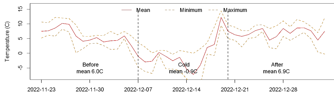
Chart 24: Temperatures before, during and after a severe cold period from 7/Dec/2022
