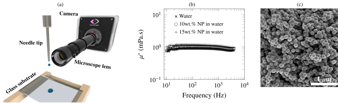
Fig. 1. (a) Experimental setup used to capture the necking during dripping and the impact of the drop on the glass substrate. (b) Viscosity measured by a PAV rheometer as a function of frequency, revealing a negligible impact of nanoparticles on fluid behavior across a range of frequencies. (c) SEM image confirming the spherical morphology and uniform size distribution of silica nanoparticles used in this study.
