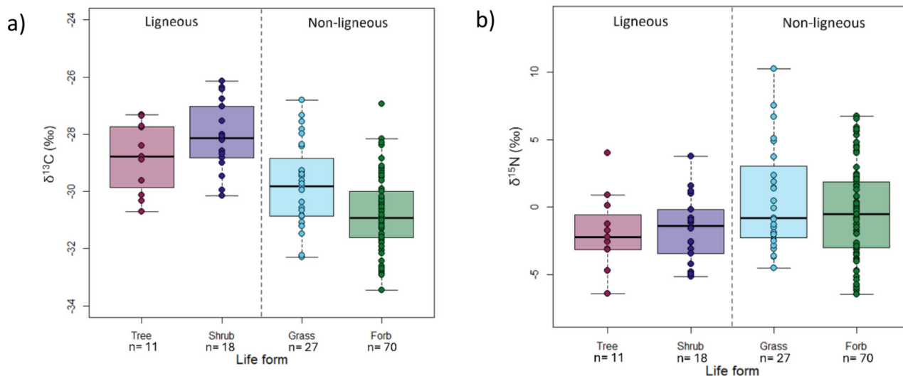
FIGURE 3 | Comparison of \delta^{13}\text{C} and \delta^{15}\text{N} values of plants by life form. (a) Box plot of plant \delta^{13}\text{C} values categorized as tree, shrub, grass, or forb. (b) Box plot of plant \delta^{15}\text{N} values categorized as tree, shrub, grass, or forb. Boxes represent the quartiles, the bold lines represent the medium, and the whiskers represent 1.5 \times the interquartile range. The points signify individual plants.
