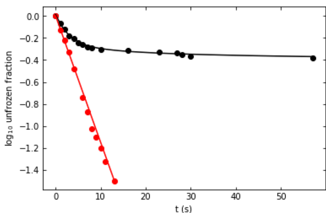
Fig. 2 Isothermal freezing data for 1\ \mu\text{L} droplets of Tris buffer containing 100\ \text{nM} annealed (well-folded) DNA origami tiles (red dots) and the same mass of unannealed origami (black dots) at -24.5\ ^\circ\text{C} . The linear fit to the annealed origami data assumes J_0 = 275\ \text{s}^{-1} and \eta = 1.0(3) \times 10^6\ \text{K}^3 (see eqn (3)). The fit to the unannealed data assumes J_0 = 0.55\ \text{s}^{-1} , \mu_\eta = 12.5 and \sigma_\eta = 3.6 (see Table S1†).
