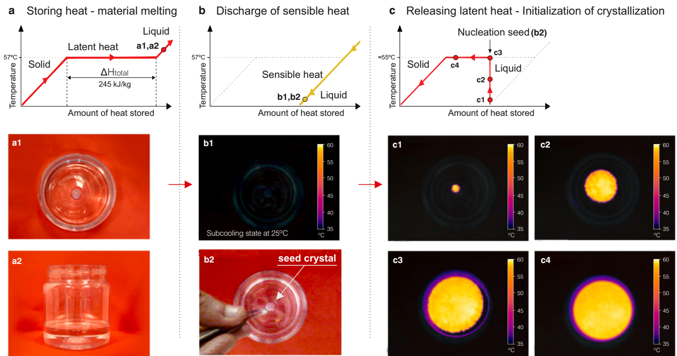
Fig. 3. Thermal energy storage process of sodium acetate (p-SA) solution with stable supercooling. a) storing heat – material melting. b) Discharge of sensible heat while latent heat is conserved and stored. c) releasing latent heat – initialization of crystallization.
