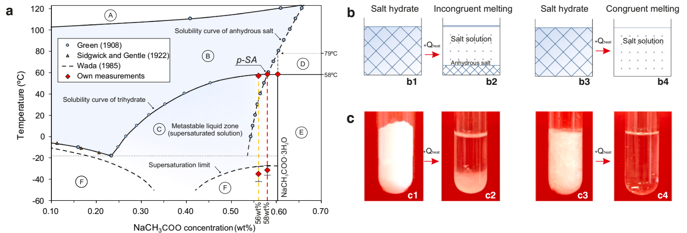
Fig. 4. Supercooling stages. a) Phase diagram of sodium acetate aqueous solution. b) Schematic sequence of the incongruent melting and congruent melting. c) Photographs of incongruent melting (SAT or SA at 60.28 wt%) and congruent melting (p-SA at 58 wt%).
