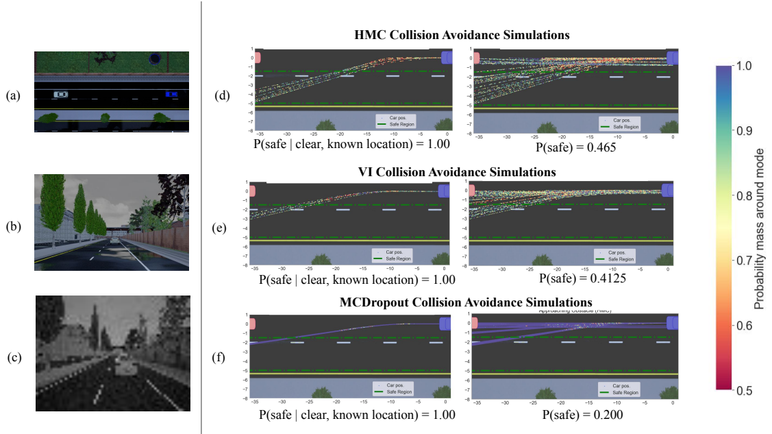
Figure 5.8: To the left of the black line, we visualize the experimental set up. (a) Spatial distribution of cars; (b) original camera signal; (c) input to BNN. In the centre of the figure we plot the course of the vehicle controlled by a BNN, where each row represents a different posterior approximation (d) HMC, (e) VI, (f) MCD. Each dot, representing the position of the car during its trajectory is colored based on the uncertainty of the controller.
