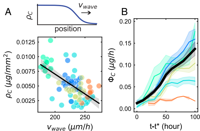
Fig. 2. Carbon expenditure pattern of various fungal strains. (A) Top: Illustration of typical fungal density wave dynamic. Bottom: Traveling-wave observables. \rho_C is the instantaneous density of carbon across the network's spatial range and v_{\text{wave}} is the instantaneous wave speed. Each small circle corresponds to an independent median of those parameters over 10 h for all plates of the same strain ( n = 7 to 11). Black line represent bootstrap regression on all datapoints. Gray shade correspond to 95% C.I. of the linear fit obtained via bootstrapping. (B) Carbon spent by the growing network in hyphal structures per hour as a function of time. The black line and shade represent average and 95% CI of all replicates' dynamics. Colored lines correspond to average and 95% confidence over all replicates for one strain. Average and 95% CI (mean \pm 2 \times s.e.m.) are computed over 10-h time intervals. For all plots, color correspondence and number of replicates are the following: R. irregularis A5 (cyan, n = 9 ), C2 (blue, n = 19 ) and C3 (red, n = 3 ), R. aggregatus (green, n = 4 ), and R. clarus (yellow, n = 4 ).
