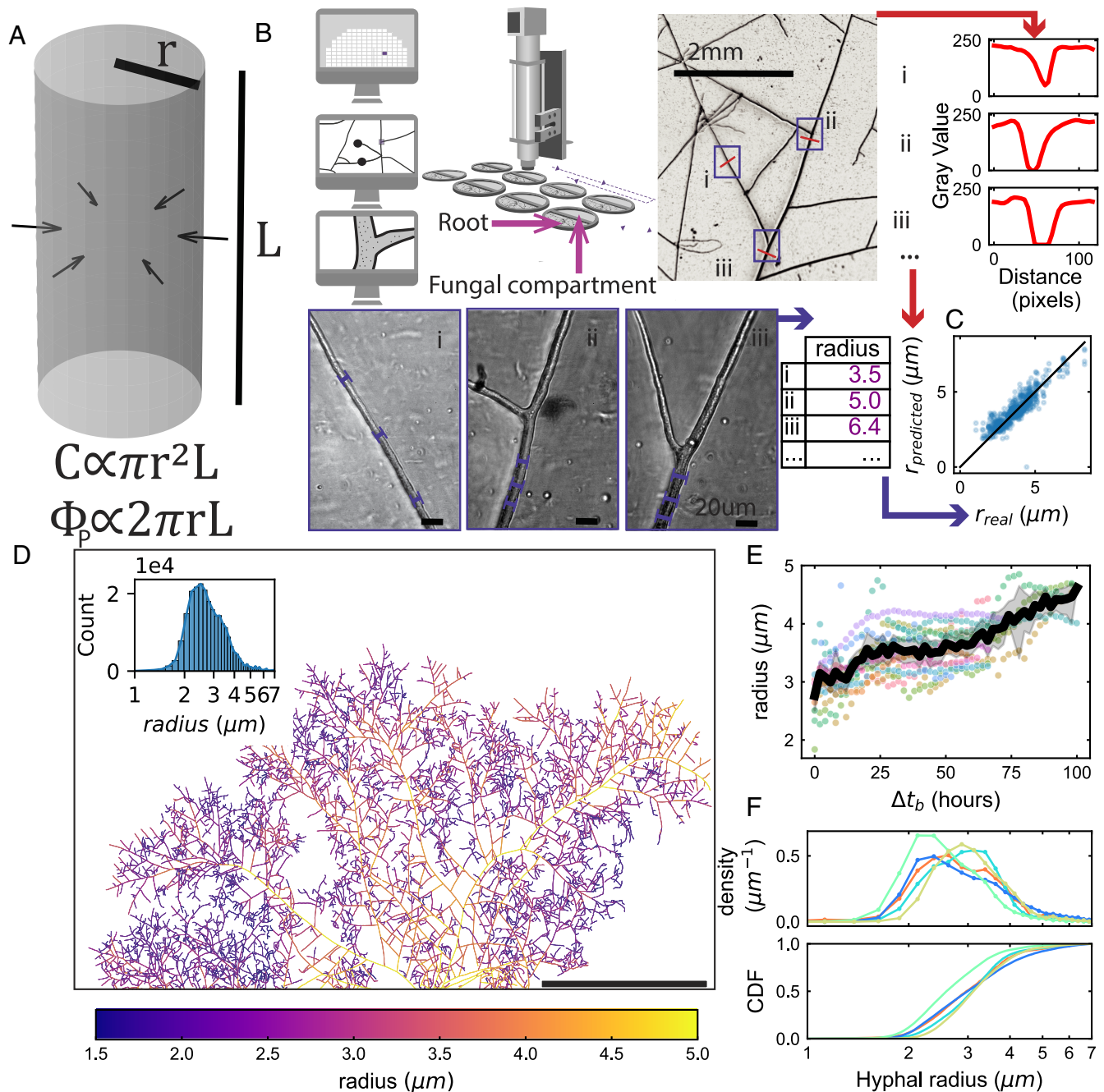
Fig. 1. Hyphal radius variation in space, time, and across genotypes as revealed by a CNN machine learning model. (A) Illustration showing the importance of hyphal radius for fungal resource economy. Cost of building a hyphal segment of length L and radius r is proportional to cylinder volume while absorption of solute from the environment is proportional to cylinder surface area. (B) Description of the dataset generation and training scheme. Images are acquired in low (scale bar is 2 mm) and high magnification (scale bar is 20 \mu\text{m} ) at different location in the network. Hyphal radius is manually measured on the high magnification images and orthogonal 120 px transect are extracted from the low magnification images. A Convolutional Neural Network (CNN) is trained to predict the measured radius from the extracted transect. (C) Evaluation of the trained neural network on an independent dataset that has not been used for training (RMSE = 0.70, R2 = 0.66). The black line is the identity function, blue points are individual predictions from the independent dataset. (D) Network graph where each edge color is mapped to the radius value estimated with the trained CNN. Inset is the distribution of radius value over all 10px segments that constitute the graph. (E) Temporal variation in radius of a selection of ( n = 13 ) major hyphae of a network as a function of the time since their emergence after branching. Each dot color correspond to a given hypha. The black line corresponds to average and gray shade to 95% CI computed on all points over intervals of two hours. (F) Upper Volume weighted distribution of the radius of all edges at final timestep for different fungal strains and species: R. irregularis A5 (cyan, n = 8 ), C2 (blue, n = 19 ) and C3 (red, n = 4 ), R. aggregatus (green, n = 4 ), and R. clarus (yellow, n = 4 ). Curves are linking the top of histogram bins. Lower Cumulative distribution function representing for each radius the proportion of total network volume that is contributed by hyphal element below that radius.
