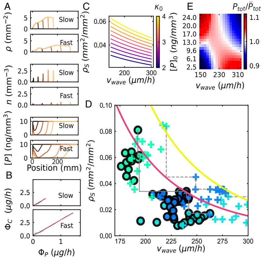
Fig. 5. Extended traveling-wave model reveals an exchange-rate-dependent Pareto front. (A) Numerical simulation results with v_{\text{wave}} = 150 \mu\text{m/h} (Upper), and with v_{\text{wave}} = 300 \mu\text{m/h} (Lower): Color gradients correspond to sampling at regular time intervals, from t = 0 \text{ h} to t = 900 \text{ h} . The first row is the hyphal length density \rho , the second row is the tip density n and last row is the P concentration [P] . (B) \Phi_C plotted against \Phi_P , during the same simulations. The red line corresponds to \Phi_C = \kappa_0 \Phi_P , the blue line corresponds to model outputs. Upper and Lower are as in (A). (C) Family of “isoexchange rate” curves computed from the analytical approximation of the traveling-wave model in the long-time limit (SI Appendix, section 3.C.3) also refer to Eq. 12, indicating a trade-off between surface area density \rho_S and wave speed v_{\text{wave}} . These curves bound from above the range of achievable AM fungal growth strategies constrained by the value of the fixed exchange rate, \kappa_0 (indicated by color). (D) Experimentally observed phenotypes in \rho_S - v_{\text{wave}} space. Data points represent median values over successive 10-h intervals in each plate, with color code as in Fig. 4. Circles, to host genotype 1; crosses, to host genotype 2. Gray lines, moving maximum of \rho_S for decreasing values of v_{\text{wave}} for each host genotype (full: genotype 1, dashed, genotype 2). Colored curves, predicted Pareto fronts computed from the analytical approximation for intermediate times when the P depletion front has yet to fully develop (SI Appendix, section 3.D) for \kappa_0 = 3 and \kappa_0 = 4 [color code as in (C)]. (E) P_{\text{tot}}/\bar{P}_{\text{tot}} as a function of wave speed v_{\text{wave}} and initial concentration [P]_0 . Color corresponds to the relative increase in total P absorption P_{\text{tot}} compared to the average \bar{P}_{\text{tot}} across each row corresponding to a given value of [P]_0 (SI Appendix, section 2.H.5).
