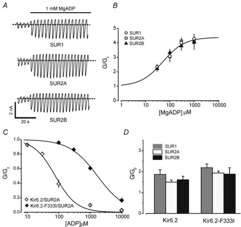
Figure 4. ADP and GDP sensitivities in the presence and absence of Mg^{2+} . A, Kir6.2-F333I/SUR1, Kir6.2-F333I/SUR2A and Kir6.2-F333I/SUR2B currents elicited by voltage ramps from -110 to +100 mV. MgADP (1 mM) was applied as indicated. B, mean relationship between [MgADP] and K_{ATP} conductance (G), expressed relative to the conductance in the absence of nucleotide ( G_0 ) for F333I plus SUR1 ( \circ ), SUR2A ( \square ) and SUR2B ( \blacktriangle ). The line is the best fit of eqn (2) ( EC_{50} = 52 \mu M , A = 4.4 ). C, mean relationship between [ADP] and K_{ATP} conductance (G), expressed relative to the conductance in the absence of nucleotide ( G_0 ), in Mg^{2+} -free solution. Kir6.2/SUR2A ( \diamond , n = 4 ) or Kir6.2-F333I/SUR2A ( \blacklozenge , n = 6 ). The lines are the best fit of eqn (1) ( IC_{50} = 80 \mu M , h = 1.2 for Kir6.2/SUR2A; IC_{50} = 1.7 mM, h = 1.0 for Kir6.2-F333I/SUR2A). D, mean conductance recorded in the presence of 100 \mu M MgGDP expressed relative to the mean of that recorded in the absence of the nucleotide, for the channels indicated. The number of patches was 4–7 in each case.
