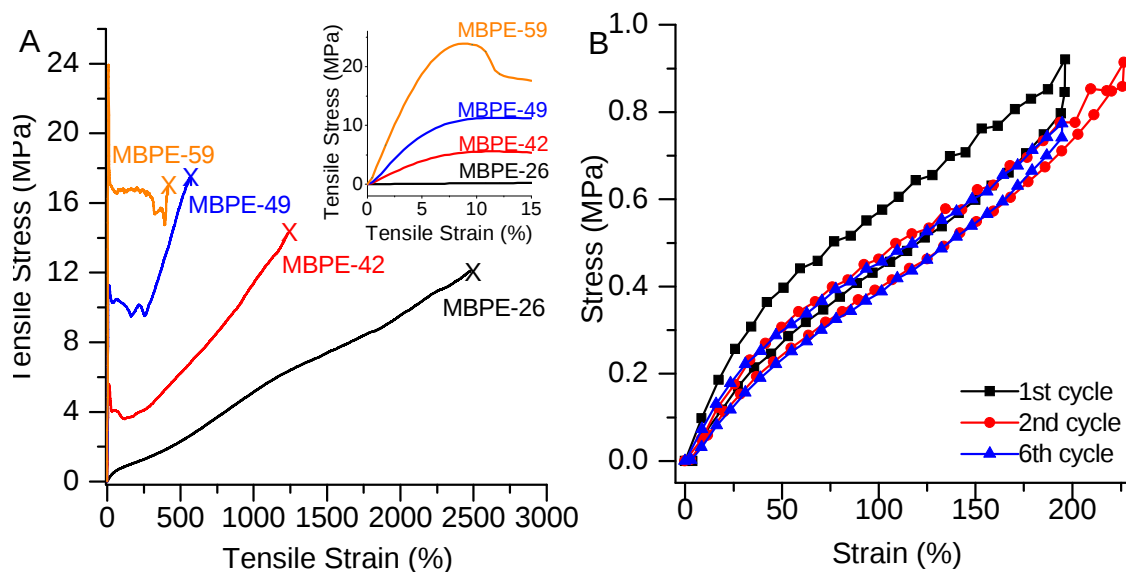
Figure 3. (A) Representative stress-strain curves for uniaxial extension of the multi-block polyesters MBPEs (Table 1). The failure points are marked with an ‘X’. Inset: enlargement of the low strain region (0–15% strain). (B) Reversible hysteresis using sample MBPE-26. The sample was tested from 0– 200% strain, over 6 cycles, at a velocity of \pm 10 mm/min. The average residual strain after the first cycle is 4 \pm 0.6\% (Table S3).
