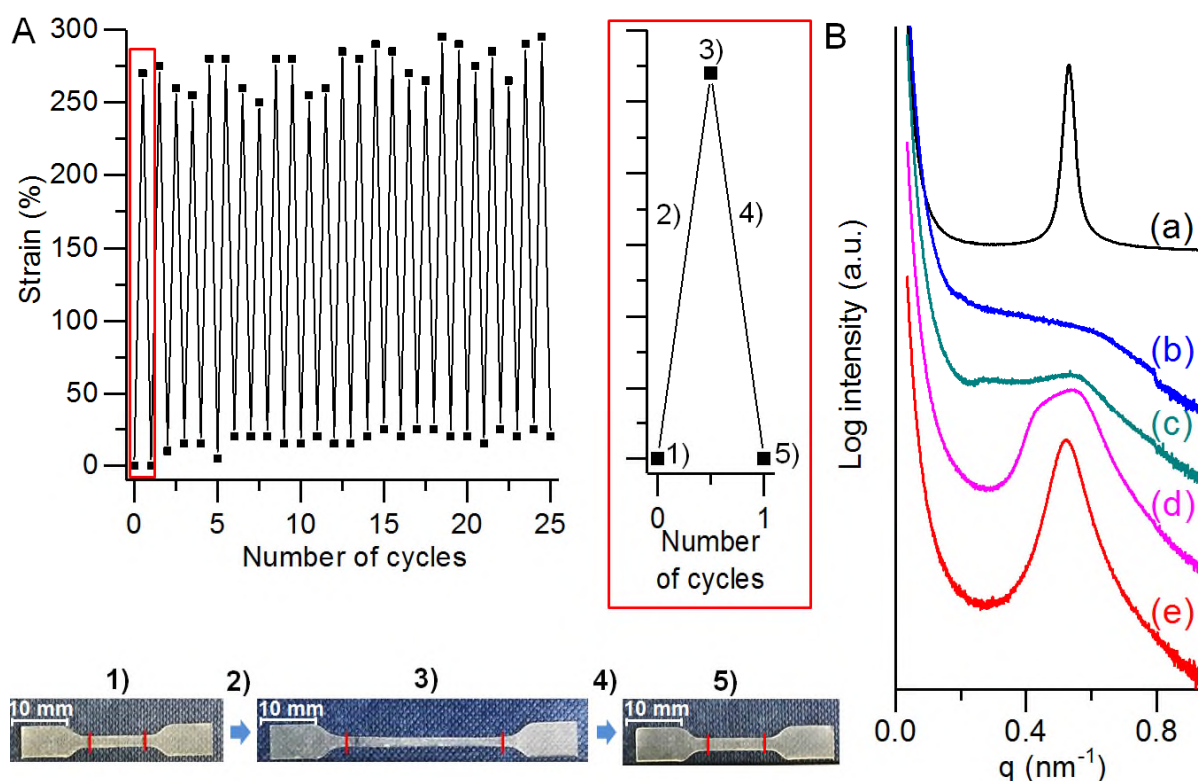
Figure 4. (A) Thermally--induced shape memory study using MBPE-59 over 25 cycles. Right: The first cycle, 1) original shape; 2) stretched to \epsilon_{\max} = 300\% ; 3) left to relax at 18 °C for 30 min; 4) heated to 55 °C to induce recovery; 5) shape recovered. Bottom: photographs of each stage of stretching and recovery of the sample. The gauge length is marked by red lines; (B) SAXS profiles of MBPE-59 during a stretching and recovery cycle. (a) as cast; (b) fully stretched ( \epsilon : 280%) at 18 °C; (c) partially recovered (residual \epsilon : 185 %) at 55 °C, 10 s, then quenched in liquid N 2 ; (d) partially recovered (residual \epsilon : 75 %) at 55 °C, 20 s, then quenched in liquid N 2 ; (e) fully recovered (residual \epsilon : ~0 %) at 55 °C, 30 s, then quenched in liquid N 2 . These samples were characterized at ambient temperature and the curves have been shifted vertically for clarity.
