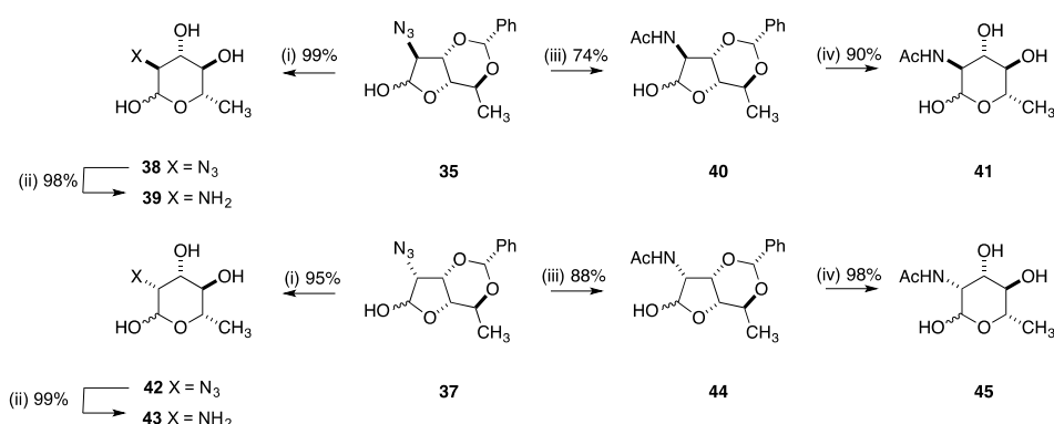
Scheme 4: (i) (\text{CF}_3\text{SO}_2)_2\text{O} , pyridine, THF, -20^\circ\text{C} , 95% (ii) \text{NaN}_3 , DMF, -40^\circ\text{C} , 75% (iii) DIBALH, \text{CH}_2\text{Cl}_2 , -78^\circ\text{C} , 3 h, 84% (iv) see text 85% 36 from 10 (v) (\text{CF}_3\text{SO}_2)_2\text{O} , pyridine, THF, -20^\circ\text{C} (vi) \text{NaN}_3 , DMF, -40^\circ\text{C} , 70% 36 and 24% 34 [over two steps] (vii) DIBALH, \text{CH}_2\text{Cl}_2 , -78^\circ\text{C} , 3 h, 87%
