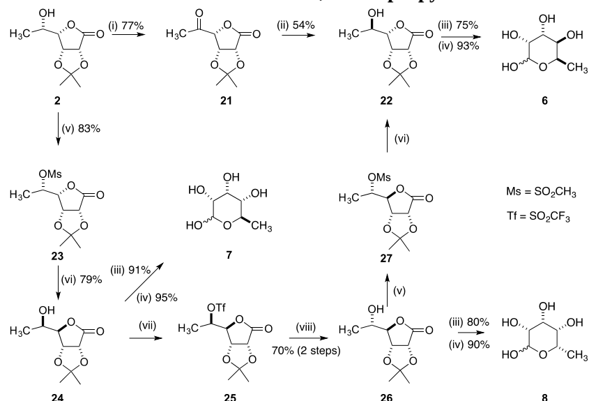
Scheme 2: (i) Dess-Martin periodinane, CH 2 Cl 2 (ii) NaBH 4 , MeOH, rt (iii) DIBALH, CH 2 Cl 2 , -78 °C, (iv) DOWEX® 50WX8-100 (H + form), H 2 O, rt (v) MeSO 2 Cl, DMAP, pyridine, 0 °C (vi) KOH, H 2 O:1,4-dioxane, rt (vii) (CF 3 SO 2 ) 2 O, pyridine, CH 2 Cl 2 (viii) CF 3 COONa, pentanone
