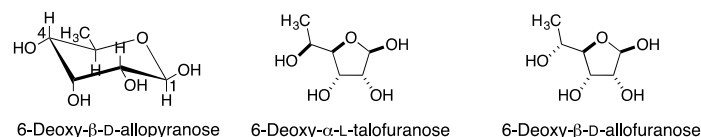
Figure 2: 6-Deoxy-β-D-allopyranose in a ^4\text{C}_1 conformation and 6-deoxy-α-L-talofuranose and 6-deoxy-β-D-allofuranose
