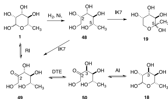
Scheme 7: (i) H 2 , Raney Ni, H 2 O (ii) IK7 (iii) RI (iv) DTE (v) AI
