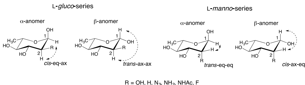
Figure 3: Conformations of 2-substituted L-quinovose and L-rhamnose
