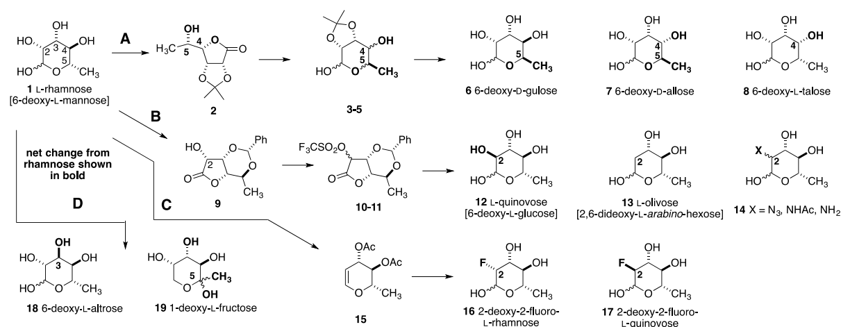
Scheme 1: Strategy for synthesis of rhamnose mimics
