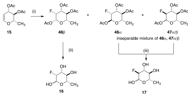
Scheme 6: (i) SelectFluor, water, MeCN; then Ac 2 O in pyridine, 27% of pure 46β (ii) CF 3 COOH, H 2 O, 100% (iii) CF 3 COOH, H 2 O, 100% (mixture of free sugars), then pure 17 was isolated by preparative HPLC
