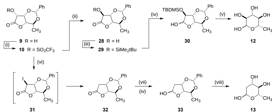
Scheme 3: (i) (\text{CF}_3\text{SO}_2)_2\text{O} , pyridine, THF, -20^\circ\text{C} , 95% (ii) \text{CF}_3\text{COOCs} , butanone, 60^\circ\text{C} , 4 h, 90% (iii) TBDMSCl, imidazole, DMF, 71% (iv) DIBALH, \text{CH}_2\text{Cl}_2 , -78^\circ\text{C} , 1 h, 88% (v) DOWEX ® 50WX8-200 ( \text{H}^+ form), \text{H}_2\text{O} , rt, 15 h, 100% (vi) \text{LiI}:\text{3H}_2\text{O} , butanone, 60^\circ\text{C} , 16 h, 74% (vii) DIBALH, \text{CH}_2\text{Cl}_2 , -78^\circ\text{C} , 3 h, 96% (viii) DOWEX ® 50WX8-200 ( \text{H}^+ form), \text{H}_2\text{O} , rt, 18 h, 100%
