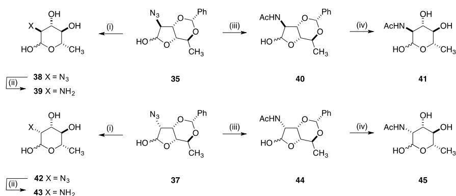
Scheme 5: (i) DOWEX® 50WX8-200 (H + form), H 2 O, rt (ii) H 2 , 10% Pd/C, HCl (iii) H 2 , 10% Pd/C, Ac 2 O, (iv) DOWEX® 50WX8-200 (H + form), H 2 O
