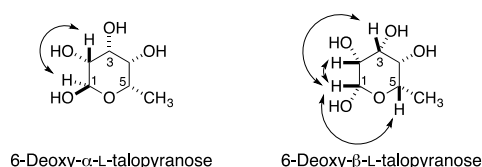
Figure 1: Key ROESY correlations of 6-deoxy- \alpha -L-talopyranose and 6-deoxy- \beta -L-talopyranose
