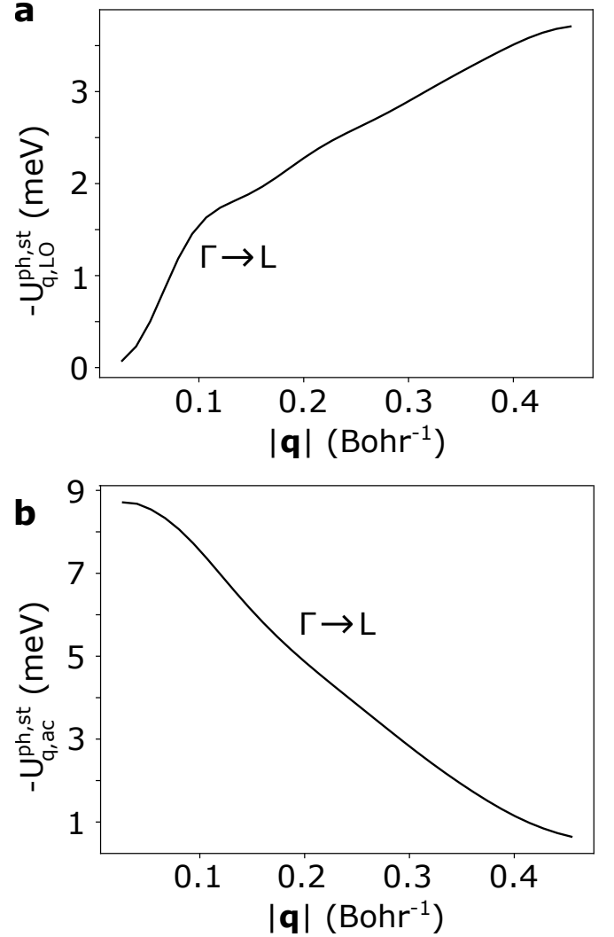
FIG. 11. Dependence of the short-range phonon-induced correction of the on-site Coulomb interaction on the phonon momentum, in the static limit. This is visualized for the LO phonon of GeTe, along the \Gamma \rightarrow L path in reciprocal space (panel a), and for the strongest coupled acoustic phonon along the \Gamma \rightarrow L path (panel b).
