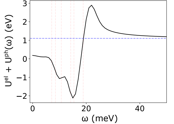
FIG. 9. Frequency-dependence of the total on-site Hubbard term for the highest-lying valence band of GeTe. The red vertical lines indicate the average phonon frequencies on the 20 \times 20 \times 20 \mathbf{q} -grid where U^{\text{ph}} is computed, while the blue horizontal line marks the value of the electronic Hubbard term of 1.102 eV for this band, in the \omega = 0 limit.
