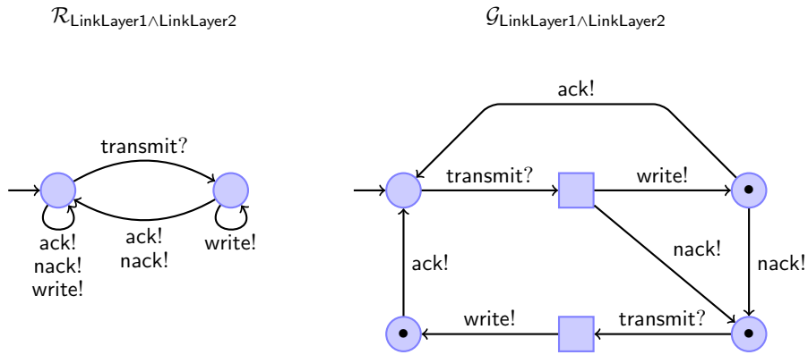
Figure 5.16: Assumption and guarantee of \text{LinkLayer1} \wedge \text{LinkLayer2}
