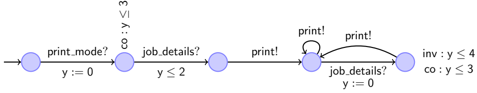
Figure 6.7: Timed disjunction of the printing/scanning and printing/faxing devices
