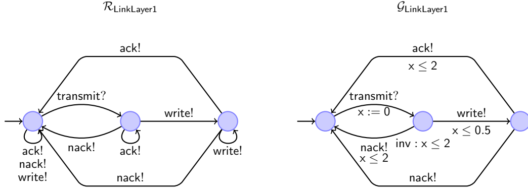
Figure 7.4: Assumption and guarantee of LinkLayer1
