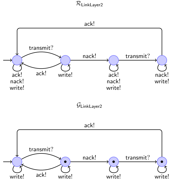
Figure 5.15: Assumption and guarantee of LinkLayer2 with restricted interface
