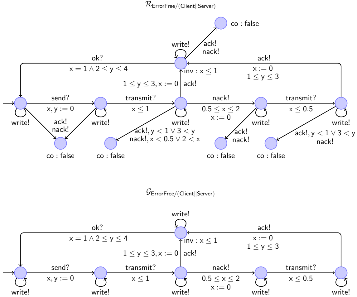
Figure 7.5: Assumption and guarantee of \text{ErrorFree}/(\text{Client} \parallel \text{Server}) with full interface
