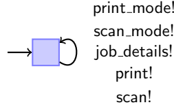
Figure 3.9: ErrorFree component
