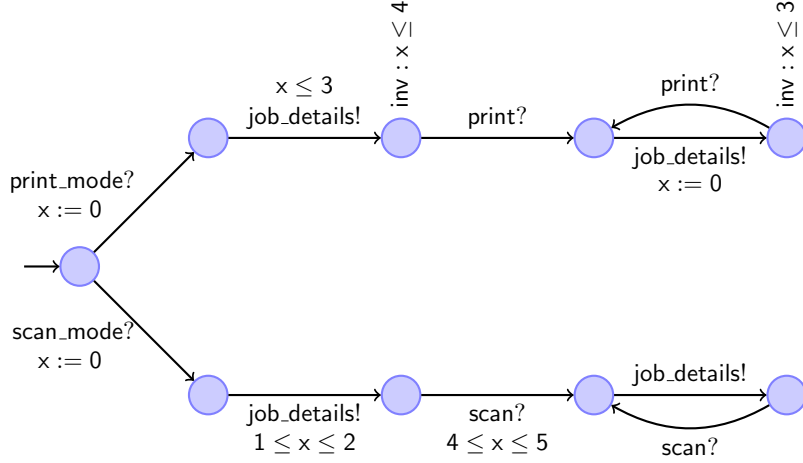
Figure 6.3: Timed spooler
