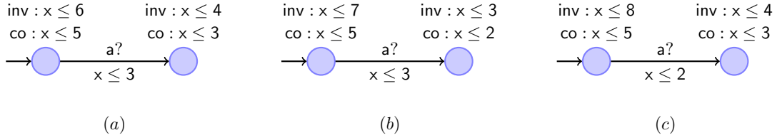
Figure 6.2: Timed refinement
