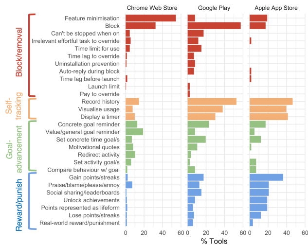
Figure 4: Functionality of digital self-control tools on Chrome Web (n = 223), Google Play (n = 86) and Apple App Store (n = 58)
