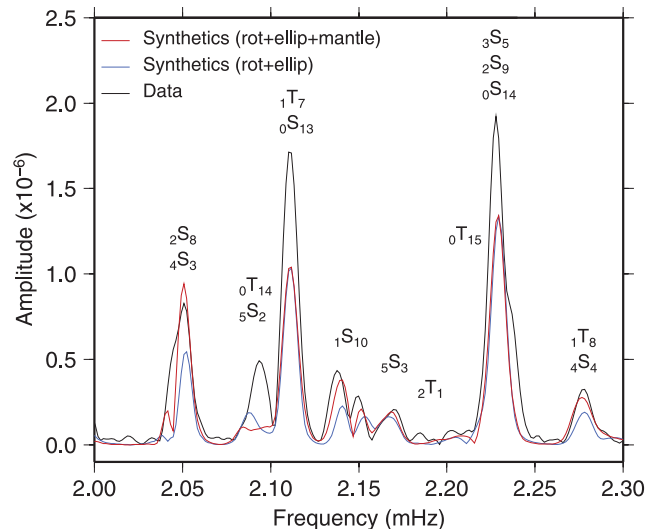
Figure 1. Amplitude spectrum of a Fourier transformed seismic record (5–70 hr) of the deep 1994 June 9 Bolivia earthquake recorded at station ATD (black) for a frequency window containing mantle sensitive modes. Synthetic data is calculated using full-coupling (Deuss & Woodhouse 2001) for rotation, ellipticity and heterogeneous mantle structure (red) and rotation and ellipticity only (blue). Theoretically predicted frequencies of normal modes are indicated.
