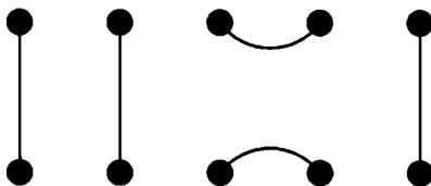
FIG. 2. The generator E_3 for r = 5 .
