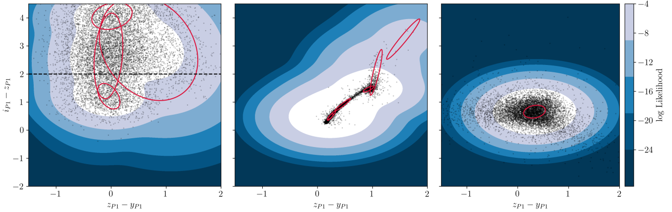
Fig. 1. Log likelihood of quasars ( left ), dwarf stars ( middle ), and low-redshift galaxies ( right ) modelled by a Gaussian mixture model in colour space. The red ellipses indicate the 3-sigma extents of the individual deconvolved Gaussians (four components for quasars, six for dwarf stars, and one for galaxies). The quasar likelihoods are assigned using photometry from simulated quasar spectra as highlighted in Sect. 3.1, whereas the photometry for dwarf stars and low-redshift galaxies are taken from their respective reference catalogues, Best et al. (2017) and Williams et al. (2018) (black dots). The dashed line in the left panel marks the commonly defined colour cut at i - z = 2.0 .
