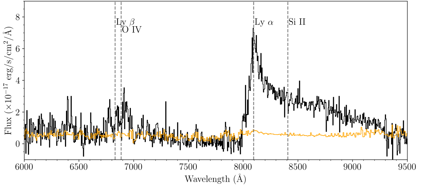
Fig. 8. 1D spectrum of P144+50 taken using the IDS instrument on the 2.5 m INT. The characteristic break blueward of the Ly \alpha line is clearly visible, unambiguously identifying it as a high-redshift quasar with a redshift of z = 5.66 based on its Ly \alpha emission. Some flux is seen around the expected Ly \beta and O IV features. Apart from Ly \alpha , there are no clear emission lines visible in the spectrum due to the limited sensitivity of the INT. The orange line indicates the noise level of the spectrum.
