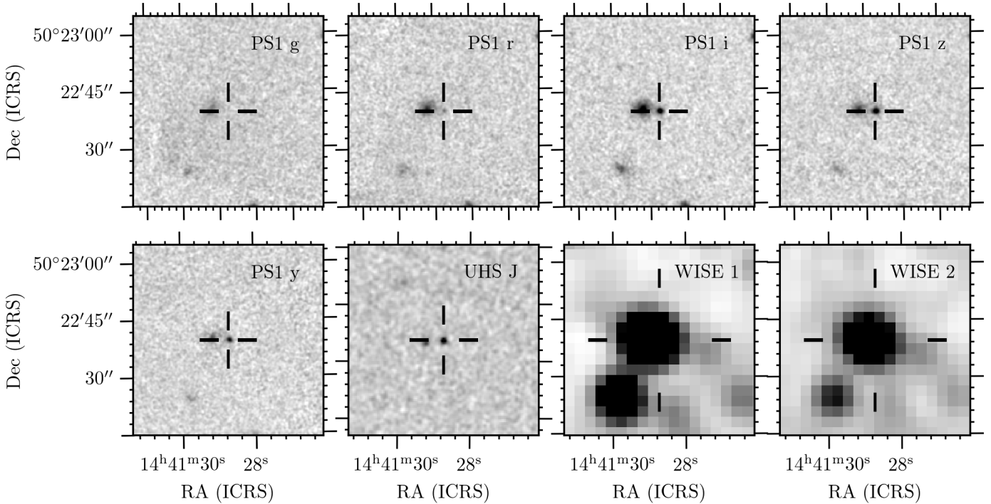
Fig. 7. P144+50 in optical and infrared bands. In the WISE images, it is blended with the neighbouring galaxy. Given the fact that the quasar is brighter in those bands while the galaxy drops off, and that its WISE magnitudes are consistent with those of other HzQs, it is likely that most of the emission in the WISE bands comes from the quasar.
