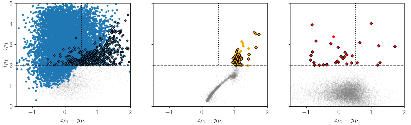
Fig. 6. Distribution of sources in the z_{P1} - y_{P1} vs i_{P1} - z_{P1} diagram of the test samples of HzQs ( left ), brown dwarfs ( middle ), and galaxies ( right ). Sources not selected with any method are marked in grey. Sources selected with i - z > 2 colour cut (dashed line) but rejected by the probability selection are marked as a diamond shape with a black edge. Notably, the z - y < 0.5 colour cut (dotted line) rejects all brown dwarfs from the test sample, but also a large portion of the simulated quasar sample.
