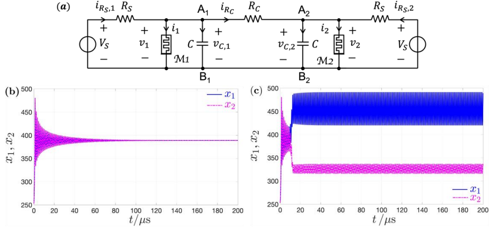
Figure 12. (a) The simplest ever-reported bio-inspired circuit, 148 which reproduces the counterintuitive diffusion-driven transition from quiescence to sustained oscillatory behavior, observed by Smale in an eight-order reaction-diffusion system from cellular biology, 149 through half the number of dynamical states, encoded in two capacitors and two locally-active NaMLab memristors, 146 on the proviso that the two identical memristive Pearson-Anson cells are preliminarily poised on some common Edge of Chaos operating point before the diffusion path, enabling their diffusive interaction, is activated. The four degrees of freedom of the proposed fourth-order RD-MCNN are encoded in the memristors' states x_1 and x_2 , and in the capacitors' voltages v_1 , and v_2 (refer to ref 148 for details). (b)-(c) Diffusion-induced transition of the bio-inspired array of (a) from silence to persistent oscillatory mode (all details on memristor model and cell parameters, chosen through a systematic methodology from Local Activity and Edge of Chaos Theory, are reported in ref 148). (b) Progressive approach of the states x_1 and x_2 of memristors M_1 and M_2 toward the same quiescent steady state, which they would independently attain, irrespective of the initial condition, in case they were let evolve in the respective uncoupled cell. Here R_C = 50 \Omega , while the initial condition for the cell i = 1(2) is arbitrarily set to (x_i(0), v_{C,i}(0)) = (253.15, \zeta \cdot 0.1 \text{ mV}) . (c) Formation of one of the two admissible dynamic
