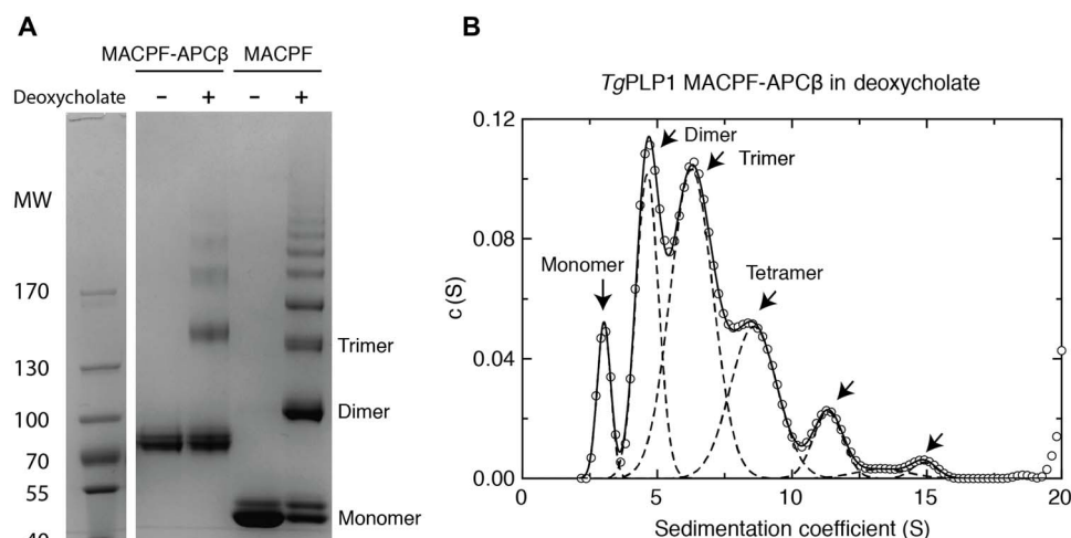
Fig. 2. TgPLP1 forms a detergent-induced oligomer. (A) SDS–polyacrylamide gel electrophoresis (SDS–PAGE) of TgPLP1 MACPF-APCβ and MACPF domain with or without detergent. (B) Analytical ultracentrifugation of TgPLP1 MACPF-APCβ (0.5 mg/ml) in detergent. The species corresponding to monomer, dimer, and other oligomers are indicated with arrows.
