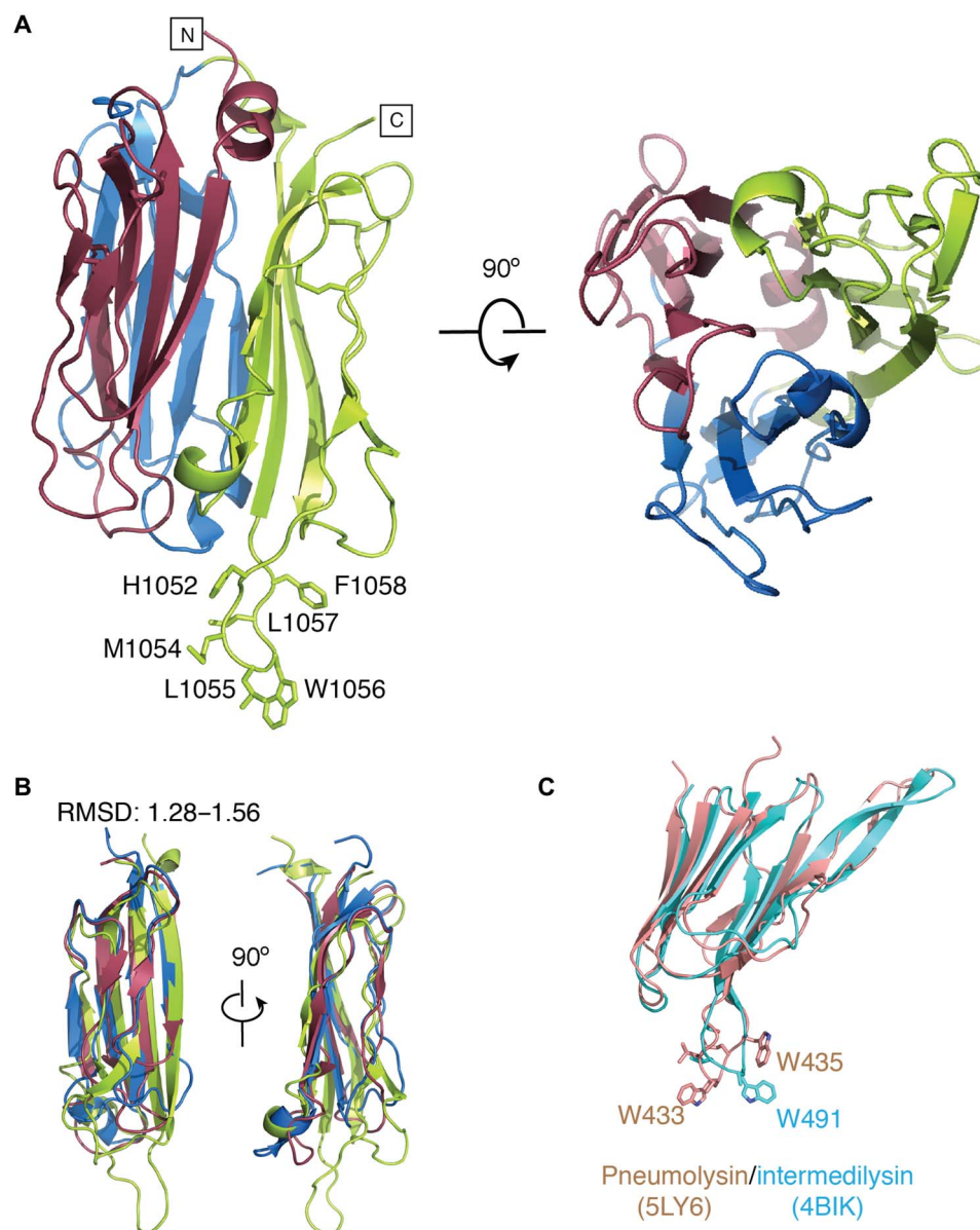
Fig. 3. Crystal structure of TgPLP1 APC \beta domain. (A) Overall structure of APC \beta domain with each repeat colored differently. Left: Side view of APC \beta domain highlighting the hydrophobic tip at the bottom. Right: Top view showing threefold pseudosymmetry with four antiparallel \beta -strands forming the core of the domain. (B) Superposition of three tandem repeats showing the conservation within the main scaffold and variation in the bottom loop of each repeat. (C) Crystal structure of pneumolysin and intermediolysin Ig-like domains, with the tryptophan hydrophobic tip highlighted.
