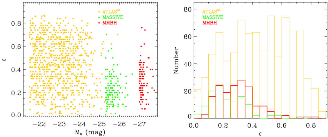
Figure 3. Ellipticity ( \epsilon = 1 - \text{sup\_ba} ) versus K_s -band luminosity (left) and ellipticity distribution (right) for our MMBH survey (red) in comparison with the MASSIVE survey (green; Ma et al. 2014) and ATLAS 3D (yellow; Cappellari et al. 2011).
