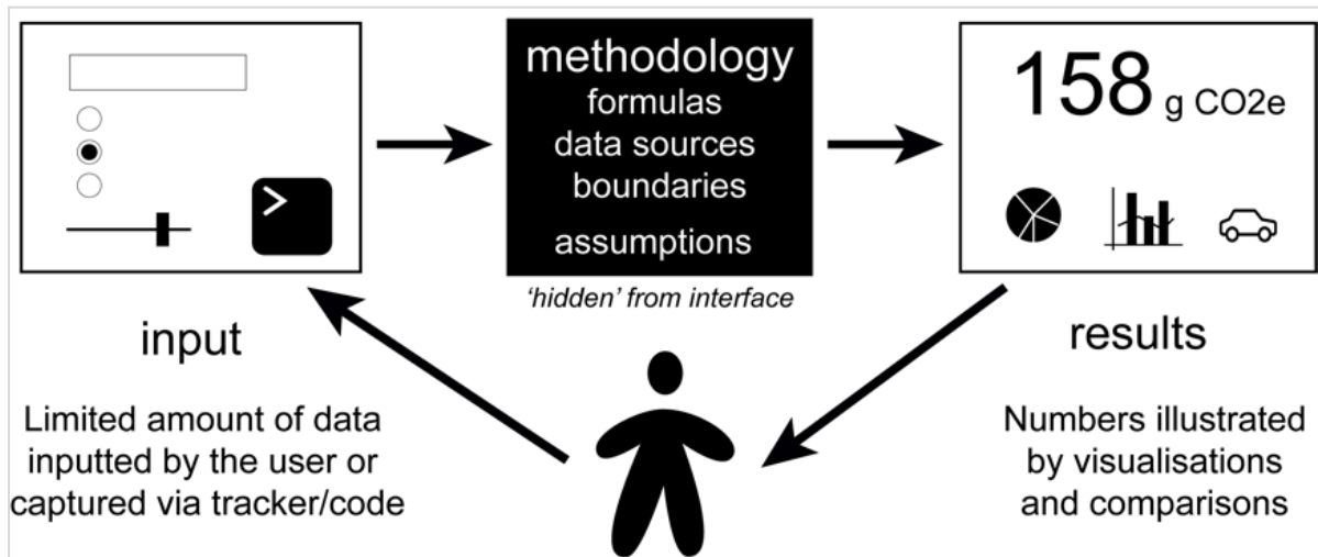
Figure 1: SEQ Figure \* ARABIC 1. A visual model of the structure of an ICT carbon calculator.
