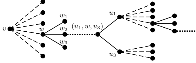
Figure 2: Example of the exploration tree \mathcal{T}_{v,t} for \ell = 3 . The children of the root vertex v are w \in C_v(F) (vertex nodes), which in turn each have children w_1, w_2, w_3 (index nodes of types 1, 2, 3). Every w_j has all (so far untested) tuples \underline{u} = (u_1, u_2, u_3) \in E_t with u_j = w as children (tuple nodes), whose descendants are component nodes u_i with i \neq j (of types 1, 2). If u_i is not already a vertex node of \mathcal{T}_{v,t} , then its children are w \in C_{u_i}(F) (vertex nodes), for which we repeat the above construction.
