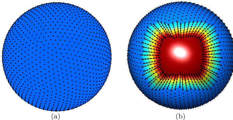
Figure 2: (a) RBF node layout on the surface of a sphere; (b) 3-D view of the discretization of the spherical shell used in the hybrid RBF-PS calculation. Blue is the outer boundary and red is the inner boundary, black circles display the computational nodes, which are distributed in the radial direction along the extrema of the Chebyshev polynomials. Note the spherical shell has been opened up in (b) to show the detail.
