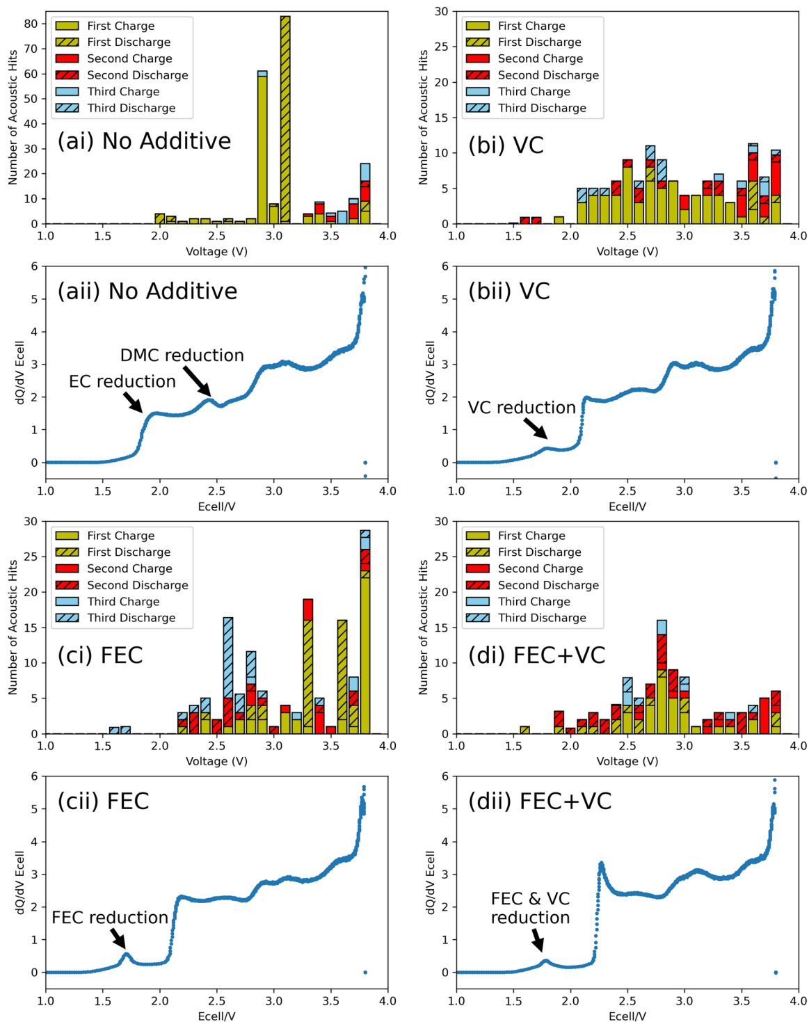
Fig. 2 AE histogram and dQ/dV plots. (ai, bi, ci and di) Number of AE hits for each charge/discharge process plotted against cell voltage in 0.1 V divisions. (a(ii), b(ii), c(ii) and d(ii)): dQ/dV from the C/20 formation cycle plotted against cell voltage. (a) No additive cell. (b) VC additive cell. (c) FEC additive cell. (d) VC and FEC additive cell for the first cycle. The dQ/dV data extracted from full-three electrode cell measurements using the same electrodes and electrolyte additives as the full pouch cells. The dQ/dV from the full pouch cells are shown in the SI (Fig. S8).
