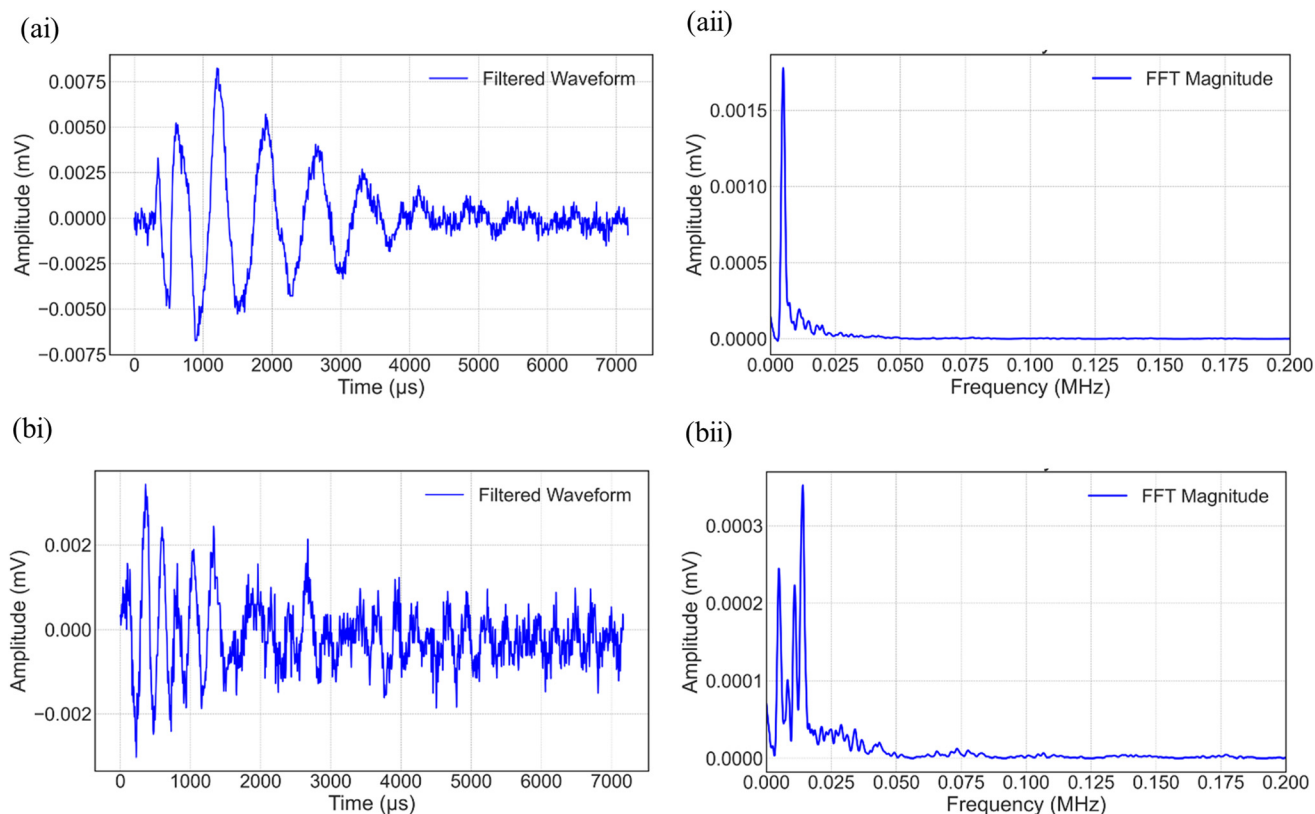
Fig. 4 Example waveforms in the time domain (ai & bi) and corresponding frequency components (a(ii) & b(ii)). Waveforms are extracted from the cell with no additive. (a) Displays a waveform produced during the first formation cycle and (b) produced later during discharge. Both signals are attributed to gassing within the cell.
