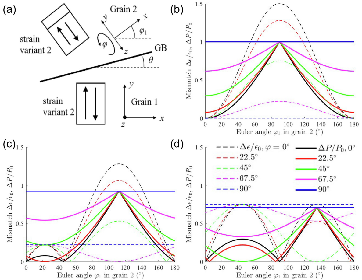
Fig. 5. Normalised strain and polarisation mismatches across a range of \phi and \phi_1 values. (a) Arrangement of domains adjacent to a GB in a lamella with three degrees of freedom indicated. (b–d) Strain and polarisation mismatches shown for various combinations of Euler angles in grain 2, with the GB angled (b) at 0^\circ , (c) at 22.5^\circ , and (d) at 45^\circ .
