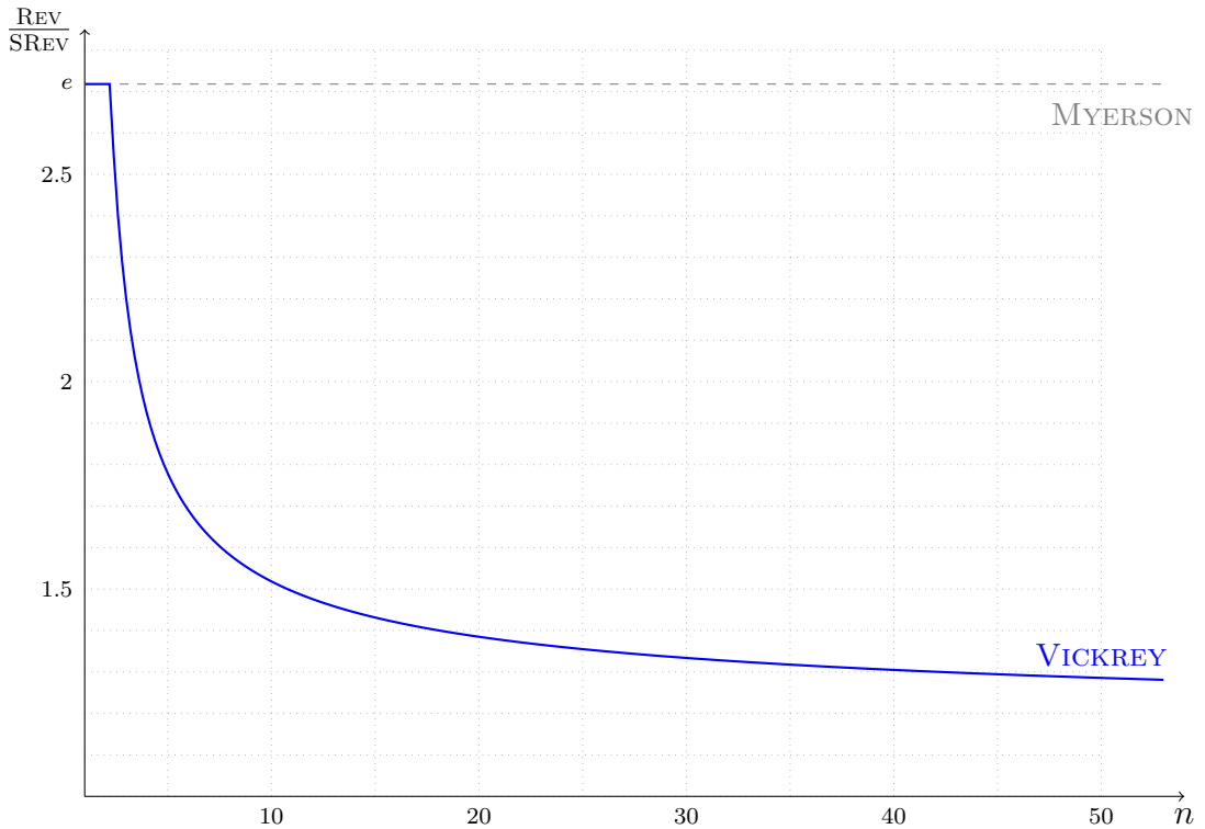
Figure 2.1: The upper bound on the approximation ratio of selling separately when the values come from independent regular distributions, as described in Theorem 2.4, drawn for n = 1, 2, \dots, 50 players (and any number of items m ). In general, an e -approximation (grey line) can be guaranteed by using Myerson’s optimal auction. In the special case of identical bidders, the analysis can be improved further by considering a simple Vickrey auction (blue line).
