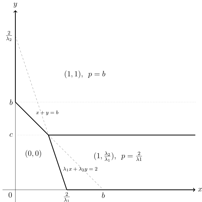
Figure A.5: The allocation function and payments of mechanism 3-RANDOM, for two exponential goods. Here b = \frac{1-W\left(-\frac{\lambda_2}{e\lambda_1}\right)}{\lambda_2} and c = \frac{\lambda_1 b - 2}{\lambda_1 - \lambda_2} .
