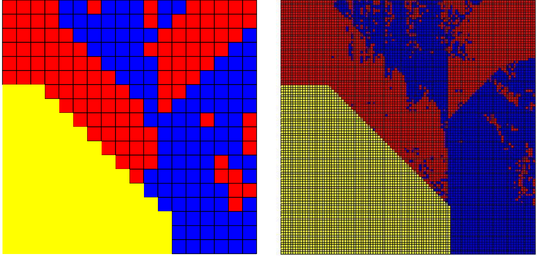
Figure 4.4: Proper colourings of the allocation space \bar{U}_\theta of the SJA mechanism for m = 2 items and different discretization factors N = 18 (left) and N = 105 (right). Blue corresponds to the direction of the horizontal axis and red to the vertical axis. The zero region U_\emptyset where no item is allocated (white region in Figure 4.2) is coloured in yellow. Notice how the entire region U_{\{1\}} is coloured blue and the entire U_{\{2\}} red. The critical and technically involved part of the colouring for two items is the one of region U_{\{1,2\}} where both items are allocated. Interpreting this in the realm of the dual program and the language of the proof of Theorem 4.3, blue is colour 1 and corresponds to the points where function z_1 increases with “full” derivative m + 1 = 3 (with respect to the coordinate x_1 ) while z_2 remains constant (with respect to coordinate x_2 ). Red is colour 2 and denotes the reverse situation where z_2 increases with derivative 3 (with respect to coordinate x_2 ) and z_1 remains constant (with respect to variable x_1 ). Yellow is colour 0 where both z_1 and z_2 are constant.
