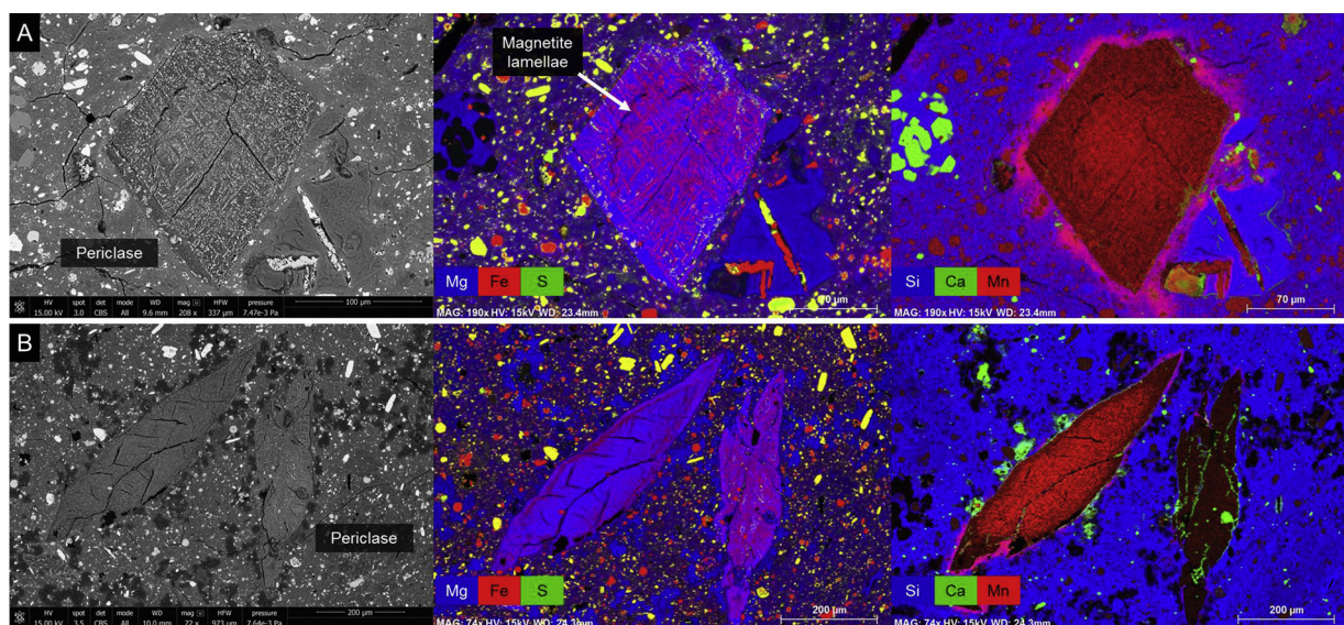
Fig. 4. BSE images (left) and corresponding EDS maps showing the distribution of Mg (B), Fe (R), and S (G) (middle), and Si (B), Ca (G), and Mn (R) (right) in periclast clasts within (a) Y-980115 and (b) Y-82162.
