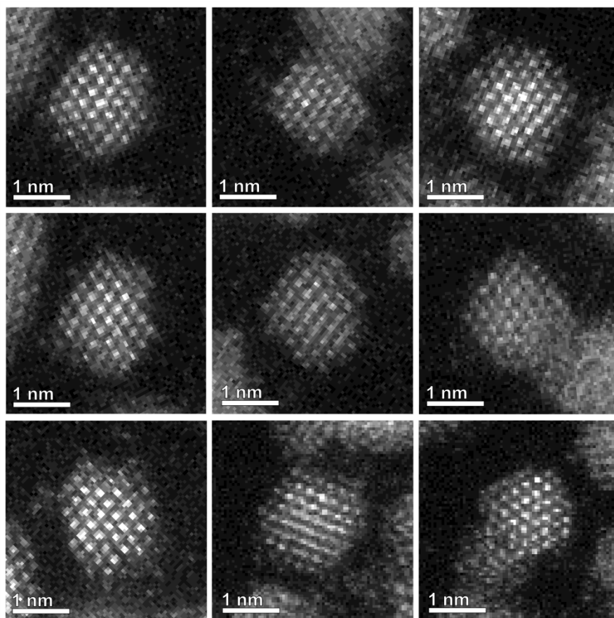
Figure S6. High resolution HAADF-STEM images of platinum nickel nuclei formed after a 7.5 second reaction time.
