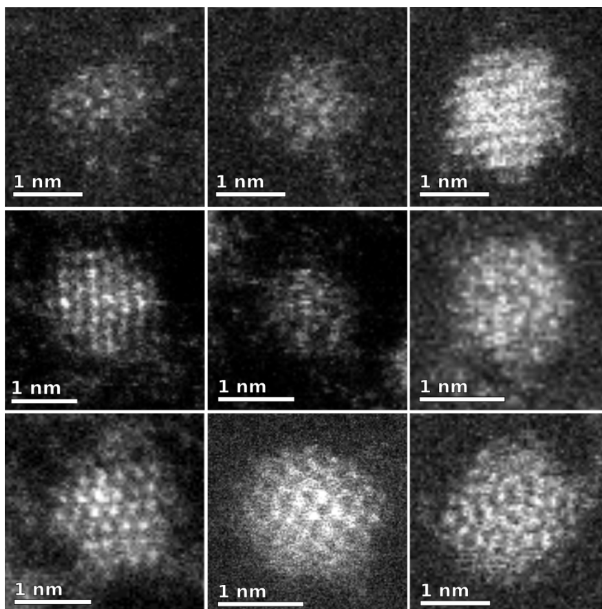
Figure S5. High resolution HAADF-STEM images of platinum nickel nuclei formed after a 5 second reaction time.
