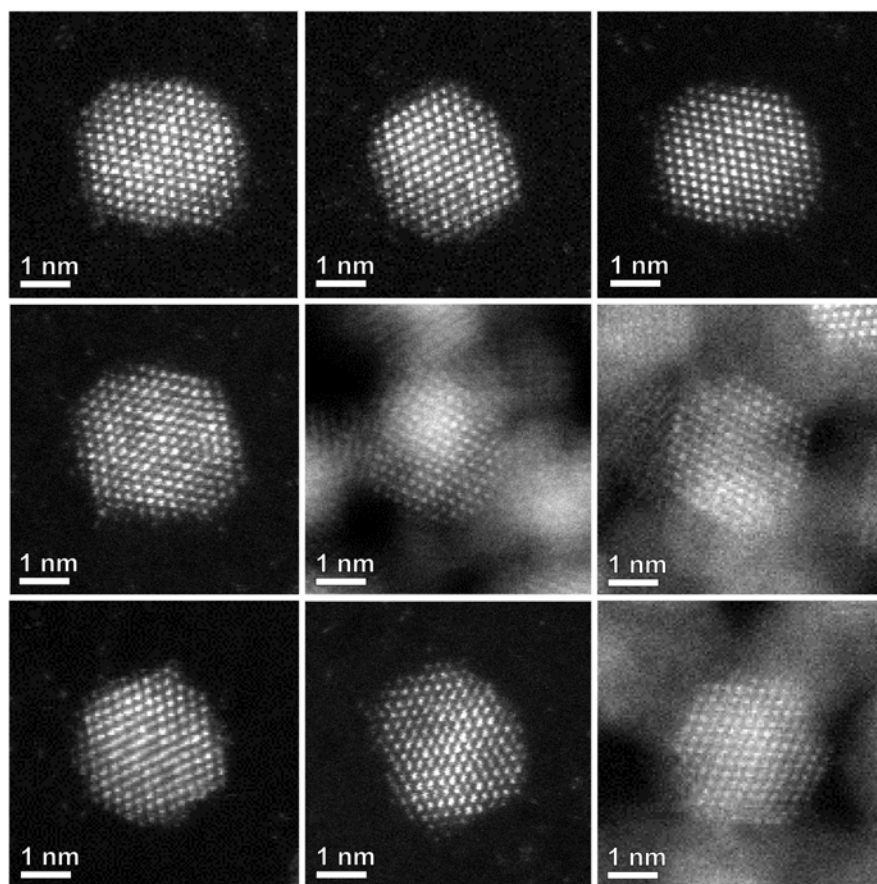
Figure S7. High resolution HAADF-STEM images of platinum nickel nuclei formed after a 10 second reaction time.
