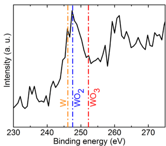
Figure S1. XPS spectra of the W 4d core levels of the left over tungsten.
