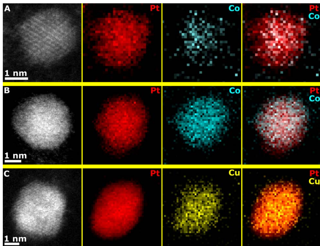
Figure S20. EELS maps of the A) 2.2 nm platinum cobalt, B) 4.0 nm platinum cobalt and a C) 3.5 nm platinum copper particle.
