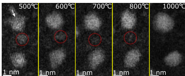
Figure S17. Platinum nickel nanoparticles from the 7.5 second sample at temperatures from 500°C to 1000°C looking at the decay of a small nanoparticle (in the dotted red circle) as the two larger particles get bigger. The white arrow shows coalescence of a small nanoparticle is shown with the white arrow.
