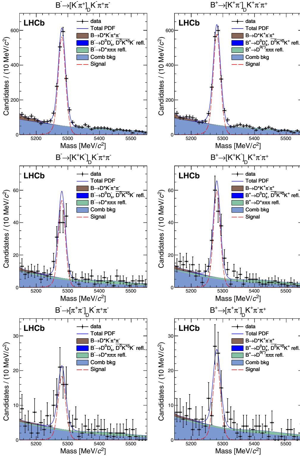
FIG. 5 (color online). Mass distributions of B^- \rightarrow DX_s^- candidates using the GLW selections, for (top left) B^- \rightarrow [K^-\pi^+]_D X_s^- , (top right) B^+ \rightarrow [K^+\pi^-]_D X_s^+ , (middle left) B^- \rightarrow [K^+K^-]_D X_s^- , (middle right) B^+ \rightarrow [K^+K^-]_D X_s^+ , (bottom left) B^- \rightarrow [\pi^+\pi^-]_D X_s^- , and (bottom right) B^+ \rightarrow [\pi^+\pi^-]_D X_s^+ .
