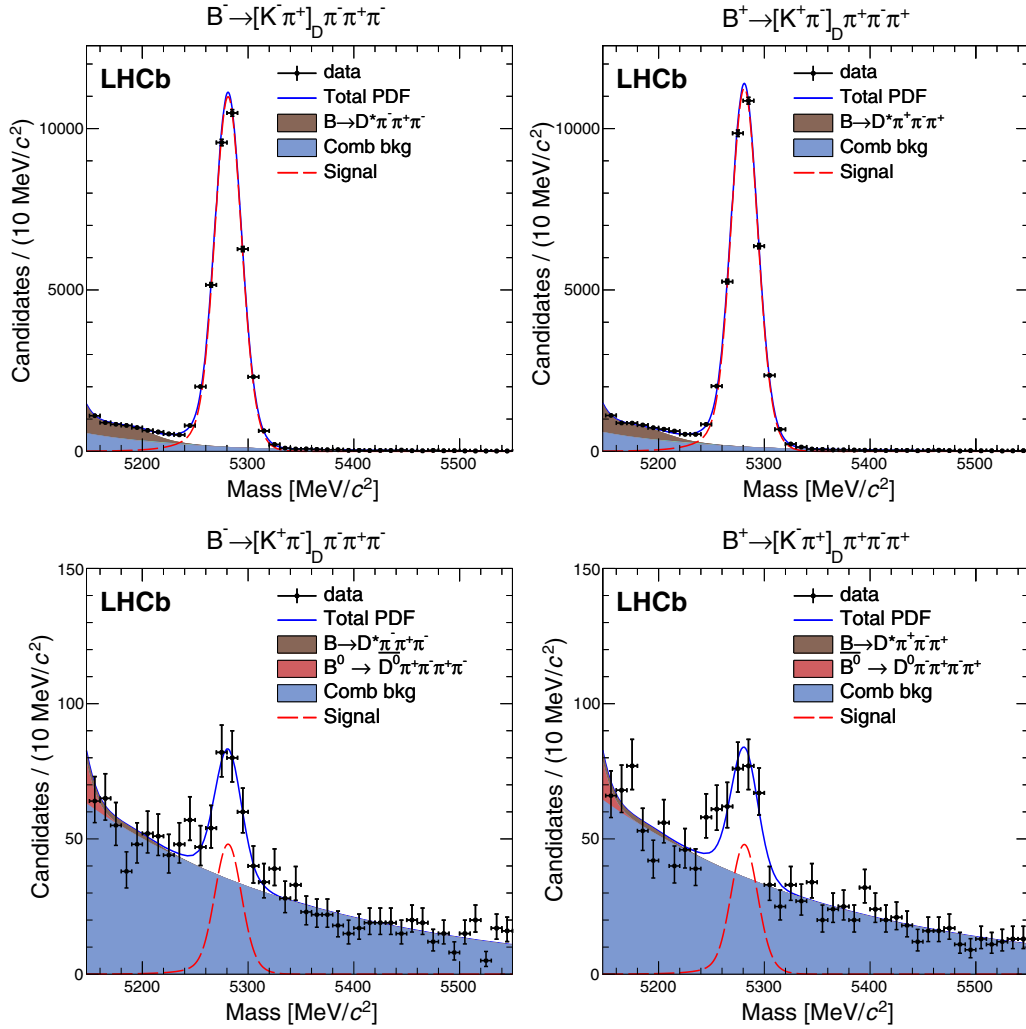
FIG. 6 (color online). Mass distributions of B^- \rightarrow DX_d^- candidates using the ADS selections, for (top left) B^- \rightarrow [K^- \pi^+]_D \pi^+ \pi^- , (top right) B^+ \rightarrow [K^+ \pi^-]_D \pi^- \pi^+ , (bottom left) B^- \rightarrow [K^+ \pi^-]_D \pi^- \pi^+ , and (bottom right) B^+ \rightarrow [K^- \pi^+]_D \pi^+ \pi^- .
