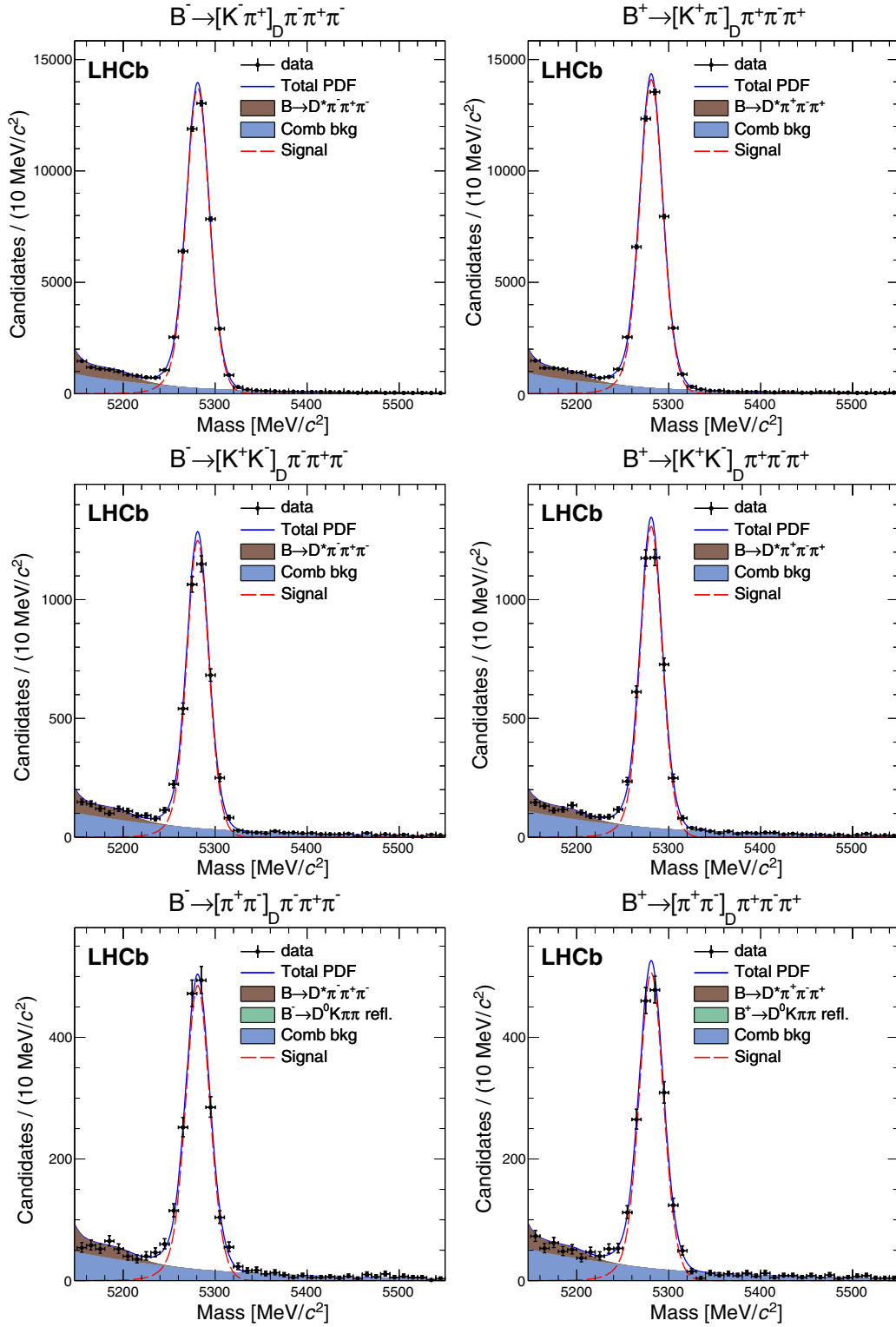
FIG. 7 (color online). Mass distributions of B^- \rightarrow DX_d^- candidates using the GLW selections, for (top left) B^- \rightarrow [K^-\pi^+]_D X_d^- , (top right) B^+ \rightarrow [K^+\pi^-]_D X_d^+ , (middle left) B^- \rightarrow [K^+K^-]_D X_d^- , and (middle right) B^+ \rightarrow [K^+K^-]_D X_d^+ , (bottom left) B^- \rightarrow [\pi^+\pi^-]_D X_d^- , and (bottom right) B^+ \rightarrow [\pi^+\pi^-]_D X_d^+
