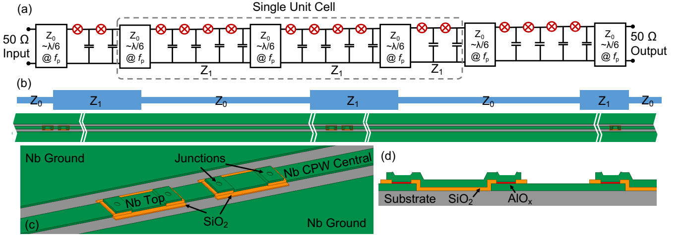
Fig. 1. (a) Circuit diagram: CPW is matched to the 50 \Omega input/output. The unit cell consists of three CPW sections and three sets of JJs where one set has fewer (or more) junctions. The total length is half the wavelength of the central frequency. (b) Schematics of the amplifier: sets of JJs are periodically embedded in the centre conductor of a 50 \Omega CPW, locally altering its characteristic impedance to Z_1 (c)&(d) Drawings show how the tunnel junction can be embedded along the CPW line. Gaps are created along the central conductor of the CPW, where thin layer of \text{SiO}_2 is deposited to protect the junction, before the top Nb layer is used to connect the CPW line.
