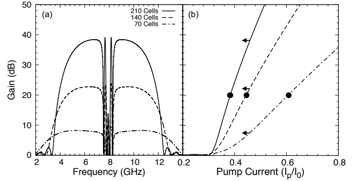
Fig. 3. (a) The gain-bandwidth product of periodically loaded JTWPAs with three different lengths: 70, 140, and 210 unit cells. The pump current is set to I_p = 0.46I_C for all curves simulated. As expected, with longer transmission length, the interaction time between the signal and the pump waves is longer, hence higher gain is achievable. (b) The parametric gain as the function of the pump current for the three different cases. The left-pointing arrows show the gain at 7 GHz, where I_p = 0.46I_C . To achieve 20 dB gain at 7 GHz, the 210-cell design requires only I_p = 0.4I_C , whereas the 140-cell design requires I_p = 0.48I_C , and the 70-cell case requires I_p = 0.64I_C .
