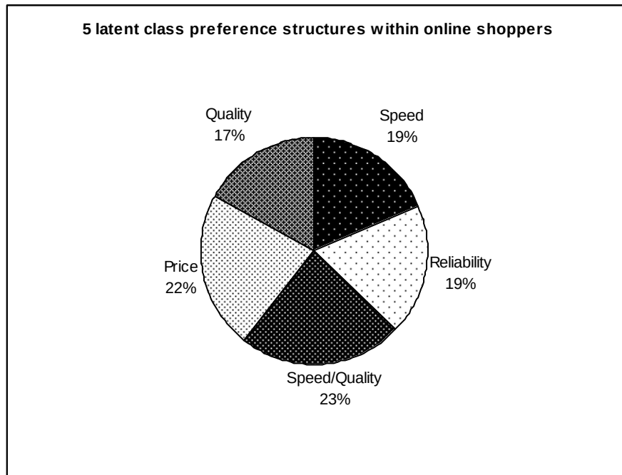
Figure 1: Share of preference between 5 latent classes
