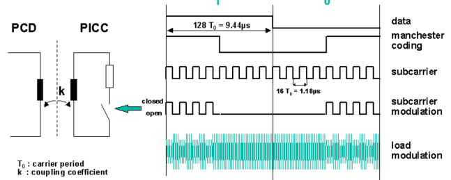
Figure 5. Manchester Encoding with Load Modulation [26]
