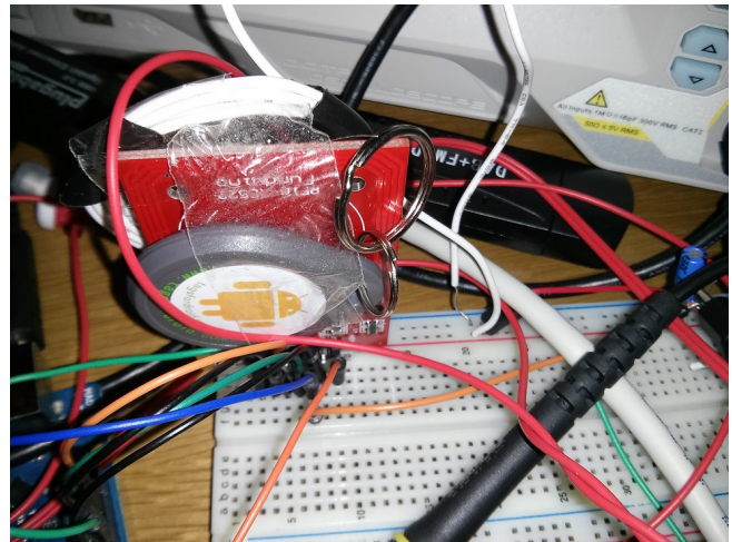
Figure 10. Setup: PICC and Antenna Attached to PCD
