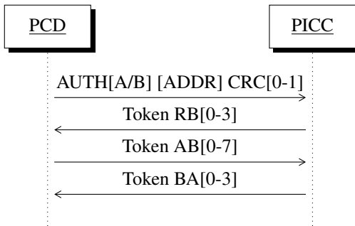
Figure 6. MIFARE Classic Authentication Protocol
