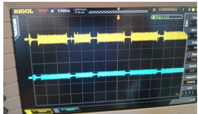
Figure 18. Reader TX in Yellow, RC522 Antenna in Blue
