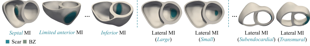
Fig. 3. Illustration of several post-MI scenarios, including different infarct locations, sizes, and transmural extents. Here, scars refer to the area of damaged or dead heart muscle tissue that has been replaced by non-functional fibrous tissue, while the border zone (BZ) is the area surrounding the scar tissue where there may be some remaining damaged heart muscle tissue that is not yet fully scarred.
