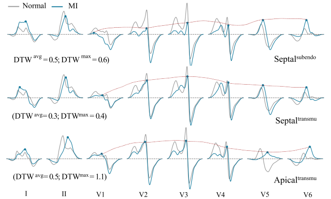
Fig. 8. Comparison of QRS morphology between MI scenarios with different transmural extents and locations, along with poor R wave progression (highlighted with red dashed lines).
