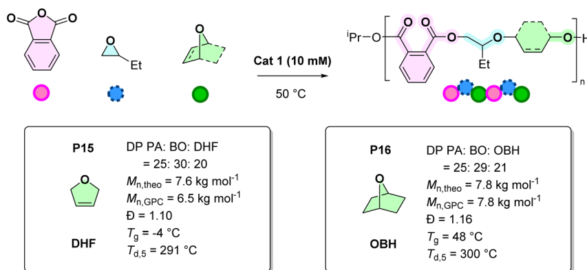
Scheme 2 Ring-opening copolymerisation (ROCOP) of PA, BO and cyclic ethers with catalyst 1 . ROCOP conditions for P15 : [ 1 ] = 10 mM, [PA] = 0.5 M, BO = 0.25 mL, 2.8 M, DHF = 0.75 mL, 9.9 M, total volume of BO + OBH = 1 mL, 50 °C. ROCOP conditions for P16 : [ 1 ] = 10 mM, [PA] = 0.5 M, BO = 0.25 mL, 2.8 M, OBH = 0.75 mL, 7.4 M, total volume of BO + OBH = 1 mL, 50 °C.
