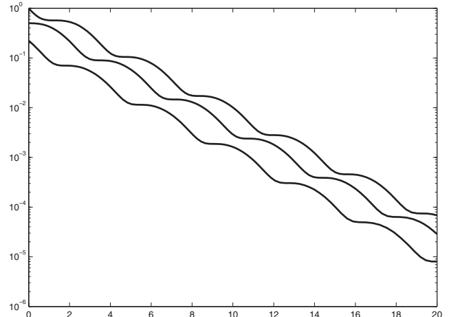
Fig. 6. A semi-log plot of \|x\| for three trajectories. We estimate \lambda = .542 for the Van-der-Pol oscillator
