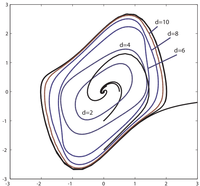
Fig. 8. Best Invariant Region vs. Degree Bound with Limit Cycle
