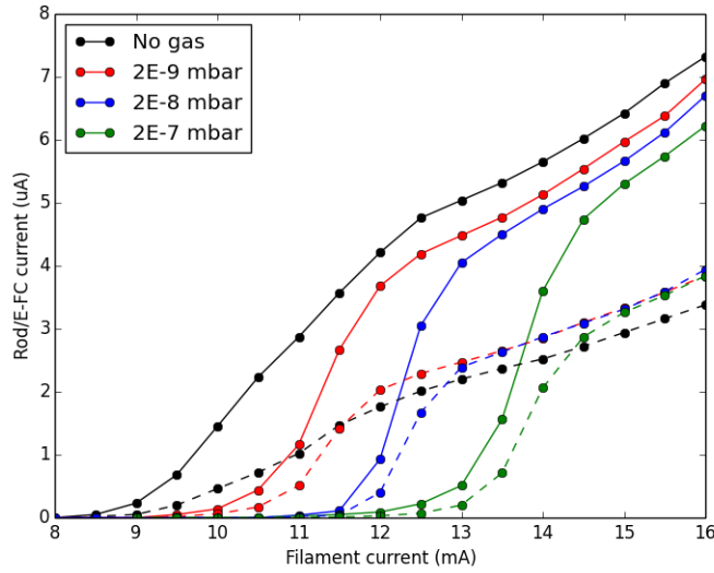
Figure 3. Variation of electron gun current as a function of filament current, measured on the electron faraday cup (dashed) and from the main rods (solid line). The output current varies with argon gas pressure.
