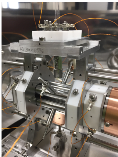
Figure 1. Close up view of the IBEX Paul trap inside vacuum vessel. The electron gun points downward between the main quadrupole rods (75 mm in length, 11.5 mm diameter), beneath which sits the electron faraday cup. To the RHS is the faraday cup and the MCP detector will be mounted on the LHS.
