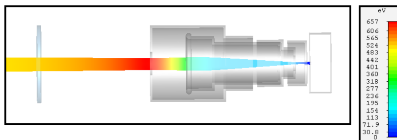
Figure 2. CST model of the IBEX electron gun in operating mode.
