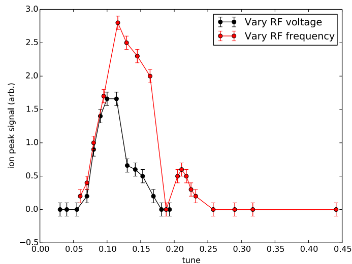
Figure 5. Variation of ion number with varying tune using either voltage or frequency to shift the operating point. The tune is the number of betatron oscillations per rf period (at 1MHz). Note that for the frequency (red) data, an additional DC bias was applied to all four rods, which increases the proportion of ions that reach the Faraday cup by providing a longitudinal velocity. Uncertainty is an estimate of oscilloscope measurement error.
