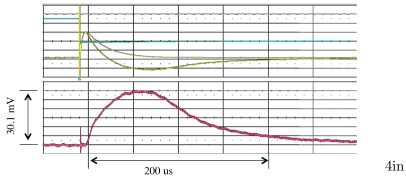
Figure 4. Oscilloscope trace of ion signal on the Faraday cup after extraction from the IBEX Paul trap. The upper trace shows timing signal (blue) and signals in yellow without (upper) and with argon gas (lower), the difference between these gives the ion signal (pink) shown on the lower trace. The noise arising from the fast gate switch can also be observed. Note that 1 mV corresponds to 0.2 nA on the vertical axis.
