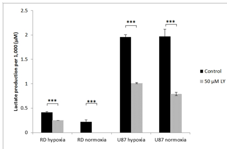
Figure 3: Lactate detected in the culture medium after 24 hours in the presence and absence of LY294002 for RD and U87 cells under 1% and 21% oxygen. The results were calibrated with relative cell number. (Using Student's t test, *** P < 0.001 ; the data are presented as the means \pm standard deviation, n = 3 )
