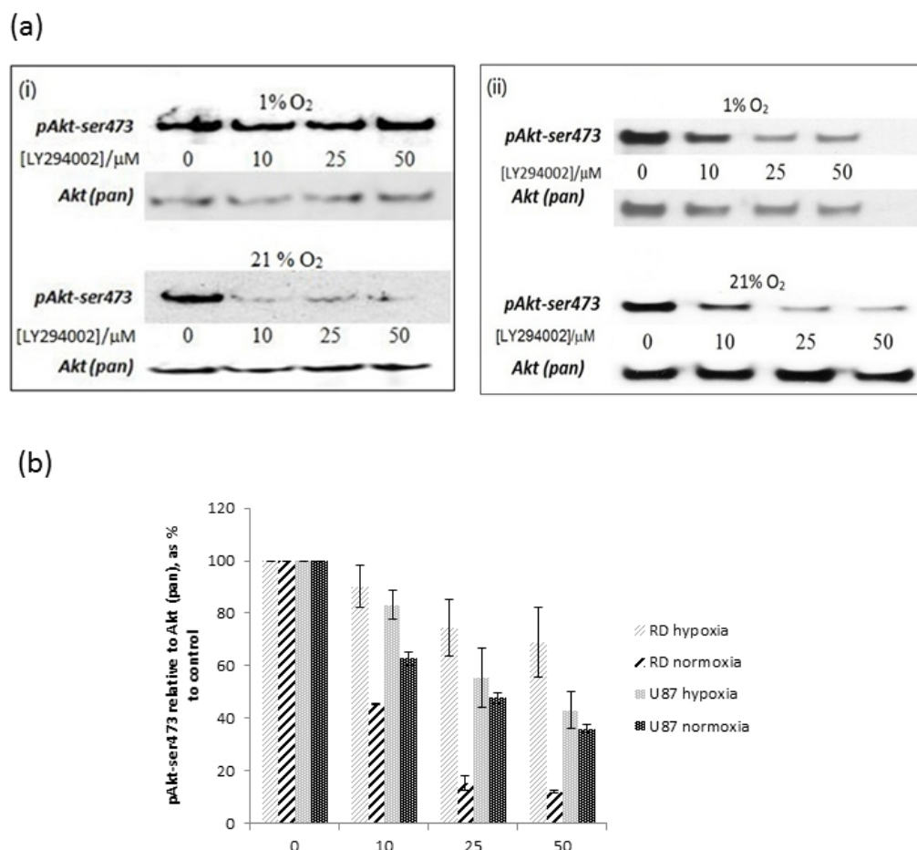
Figure 4: (a) Representative immunoblot of cell lysates from cells incubated with increasing amounts of LY294002 under either 1% \text{O}_2 (i) RD cells (ii) U87 cells. Blots were probed with anti-Akt (pan) or anti-pAkt-ser473 antibodies (b) Densitometry data taken from immunoblots shown in panel 'a'.
