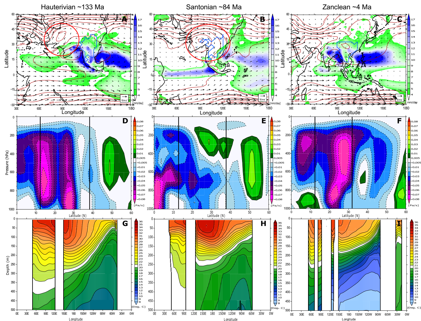
Fig. 2. Atmosphere-ocean dynamics of three key periods. Wettest month 500-mbar geopotential height (isolines), wind field (black arrows), and precipitation in the Hauterivian (A), Santonian (B), and Zanclean (C) (paleo-rotated region in blue line). Wettest month zonal cross-sectional (0°N to 60°N, 105°E to 112.5°E) vertical velocity in the Hauterivian (D), Santonian (E), and Zanclean (F) depicting the position of the Hadley circulation; negative values indicate vertical ascent, positive values indicate vertical descent, and vertical black lines depict maximum and minimum latitudinal extent of rotated EAM region. Mean annual meridional (10°S to 10°N) depth profile ocean temperature (°C) for the Hauterivian (G), Santonian (H), and Zanclean (I) depicting the location of the Pacific warm pool. Red circles denote region of interest highlighted in the main text.
