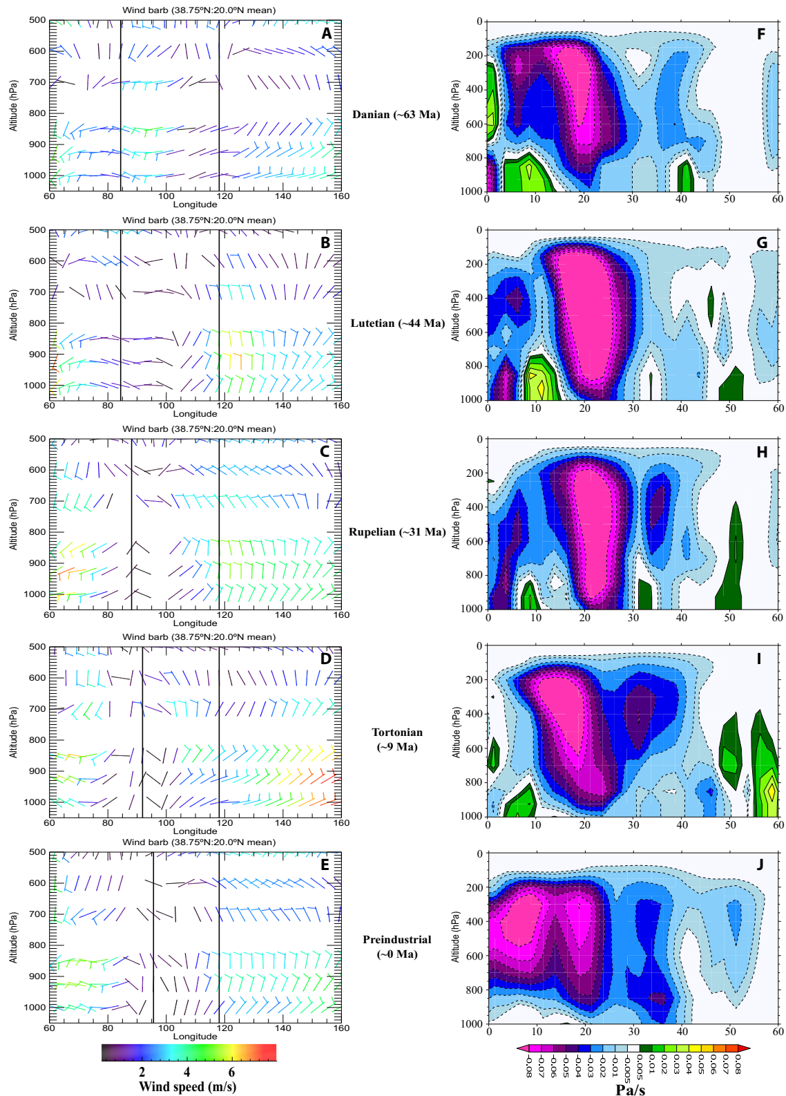
Fig. 3. EA summer (June–August) sea-breeze and maximum Hadley circulation extent. Zonal (June–August) sea-breeze circulation (left-hand column) indicated by wind barbs showing direction and magnitude (m/s; color scale) for the Danian (A), Lutetian (B), Rupelian (C), Tortonian (D), and preindustrial (E). Vertical black lines depict the maximum and minimum longitudinal extent of the EAM region (mean, 38.75°N to 20.0°N). Meridional vertical velocity (Pa/s; right-hand column) cross section (mean, 105°E to 112.5°E) in the EAM region showing the maximum northerly extent of the Hadley circulation in the boreal summer. Negative values indicate vertical ascent, while positive values indicate vertical descent for the Danian (F), Lutetian (G), Rupelian (H), Tortonian (I), and the preindustrial (J).
