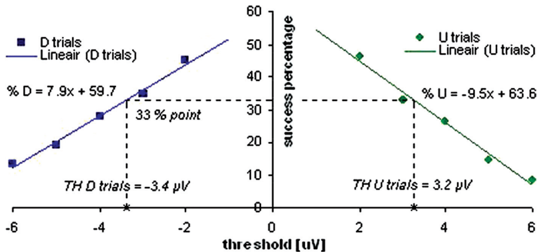
Figure 3. Example of individual threshold settings by linear regression.
