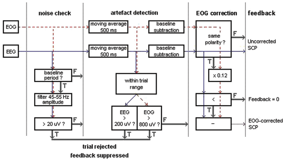
Figure 2. The detailed overview of the core of real-time data processing.
