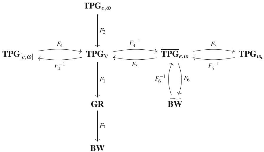
Fig. 1 Functorial relationships between categories used in this article (modelled on Nguyen et al., 2018, fig. 2).
