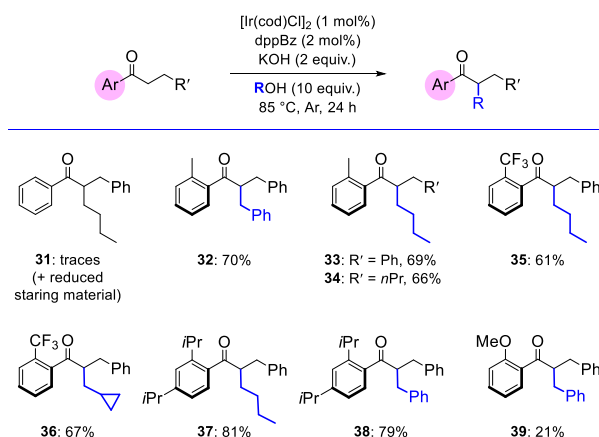
Scheme 5. ortho -Substituted aryl ketone substrate scope.
