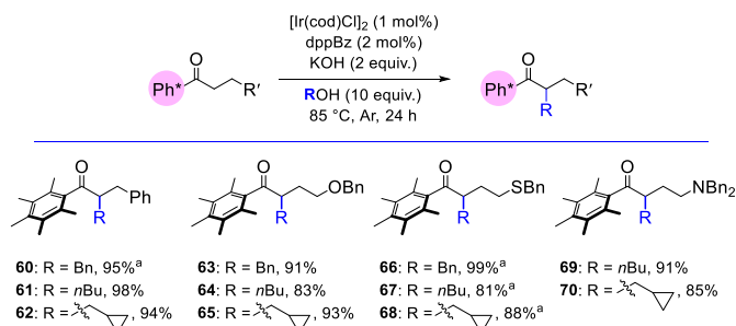
Scheme 8. Ph* ketone substrate scope.
