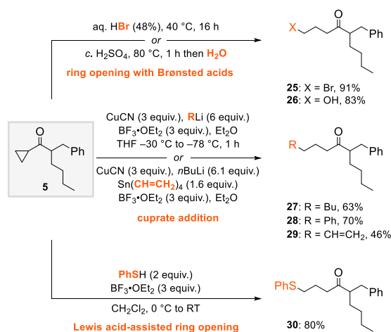
Scheme 4. Ring opening of \alpha -alkylated cyclopropyl ketones.
