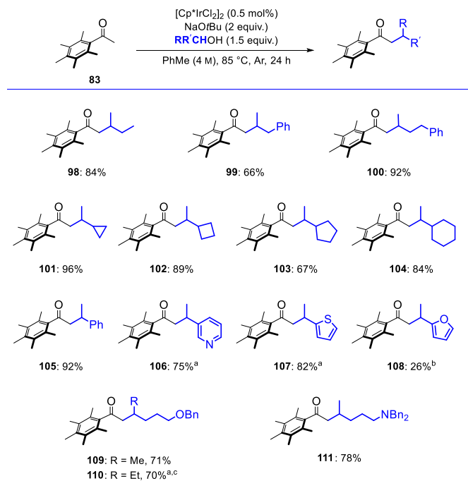
Scheme 12. Acyclic 2° alcohol scope.
