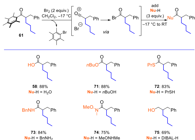
Scheme 9. \text{Br}_2 -mediated cleavage of Ph* and subsequent derivatization of the acid bromide with various nucleophiles.
