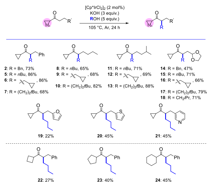
Scheme 2. Cycloalkyl ketone substrate scope.
