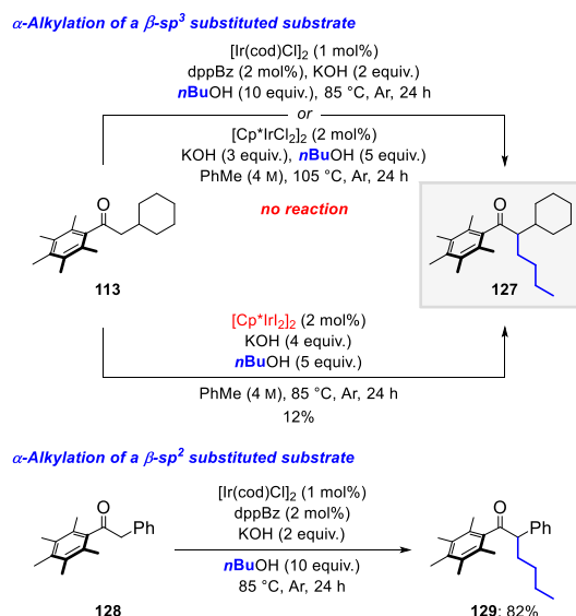
Scheme 14. \alpha -Alkylation of \beta -substituted substrates.
