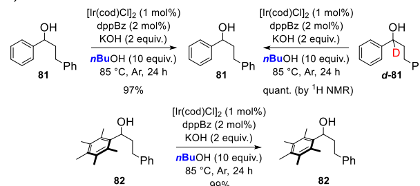
Scheme 10. Subjection of various \alpha -branching intermediates to the optimized hydrogen borrowing conditions.
