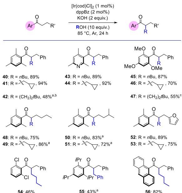
Scheme 6. Di- ortho -substituted aryl ketone substrate scope.
