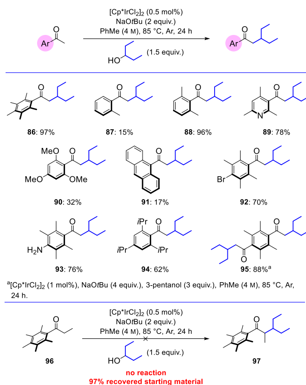
Scheme 11. Di- ortho -substituted aryl ketone substrate scope.
