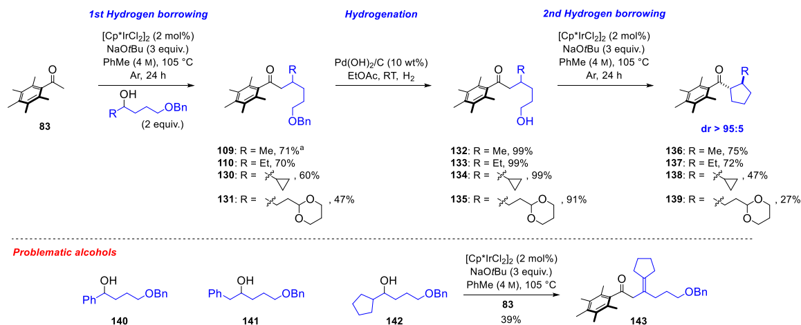
Scheme 15. Intramolecular hydrogen borrowing reaction for the synthesis of 1,2-disubstituted cyclopentanes.
