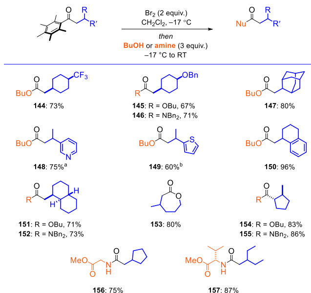
Scheme 16. Br 2 -mediated cleavage of Ph* to give the corresponding Bu ester or amide variants.
