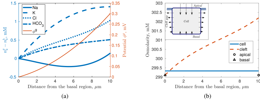
Figure 4. (a) Left axis: Deviation of the ion concentrations along the cleft from those in the basal region for the reference parameters in table 2. The x -axis goes along the symmetry mid line ( y = 0 ) of the cleft, from the basal region to the tight junction. Right axis: electrical potential along the x -axis in the cleft. (b) Osmolarity distribution along the cell ( y = H/2 + h ) and cleft ( y = 0 ). The osmolarity in apical and basal regions are shown with a circle and a triangle, respectively. Inner figure: schematic representation of the direction and magnitude of water fluxes across cell membranes.
