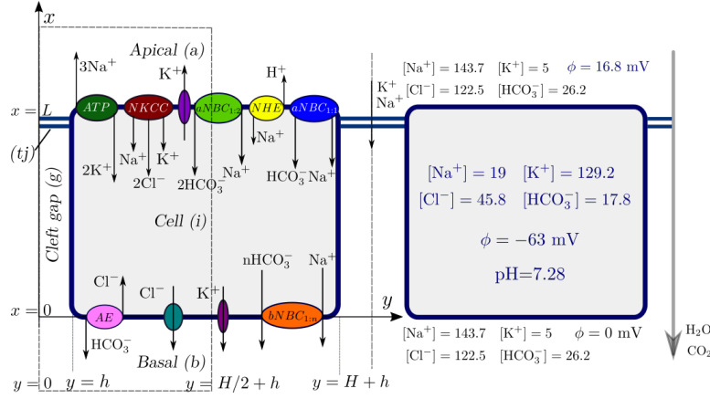
Figure 2. Left cell: Diagram of ion channels in the RPE cell membranes, with a sketched of the domain and coordinate system. Right cell: Typical values for species concentrations (in mM) and electrical potential (mV) under the open circuit condition. The prescribed values are in black and the values predicted by the model are in blue for the reference parameters of table 2, with identical concentration of CO_2 in the apical and basal regions.
