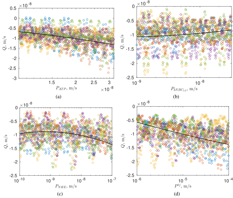
Figure 6. Scatter plots for water flux Q vs four parameters with largest sensitivity indices: (a) P_{ATP} , (b) P_{bNBC_{1,2}} , (c) P_{NHE} and (d) P^{ij} . Each point corresponds to a numerical experiment. Different colours correspond to different searching curves.
