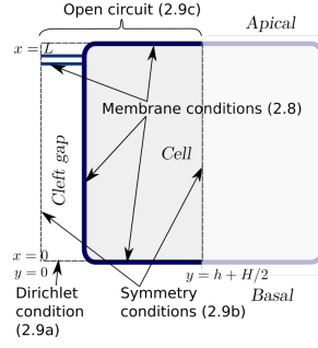
Figure 3. Sketch of the imposed boundary conditions.
