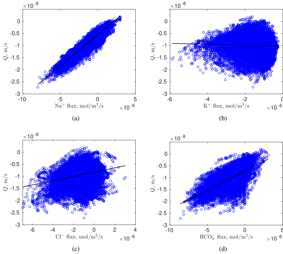
Figure 8. Scatter plots for water flux Q vs (a) \text{Na}^+ , (b) \text{K}^+ , (c) \text{Cl}^- and (d) \text{HCO}_3^- flux. Each point corresponds to a numerical experiment.
