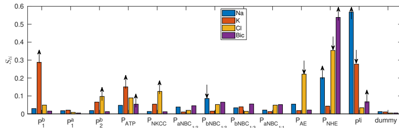
Figure 7. Total sensitivity index for ion fluxes. The arrows indicate the direction of ion flux change with the increase of a given parameter.
