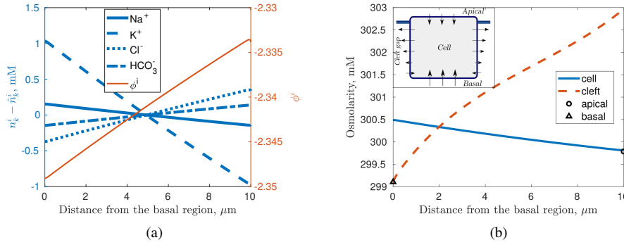
Figure 9. The case of apical \text{CO}_2 of 7% and basal \text{CO}_2 of 5%. (a) Left axis: Deviation of ion concentrations from their average value in the cell along x -axis, \hat{n}_k^i = \int_0^L n_k^i dx / L . Right axis: electrical potential along the x -axis in the cell. (b) Osmolarity distribution in the cell, cleft, apical and basal regions. Inner figure: schematic representation of the direction and magnitude of water fluxes across cell membranes.
