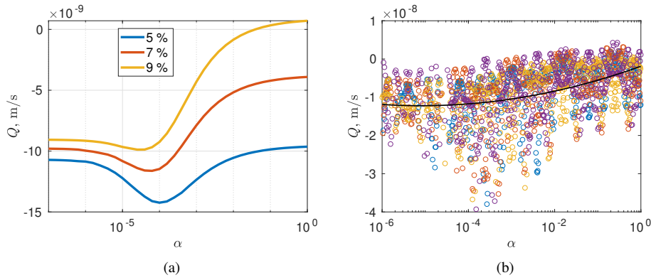
Figure 10. Water flux as a function of the CA activity. The values of \alpha on the x-axes are factors that multiply the reaction rates k_d and k_h of the reaction (2.1). The value \alpha = 1 corresponds to full catalysis (the reaction rates from table 2); as the value of \alpha decreases the catalyser is progressively inhibited. In (a) the typical solution, with other parameter values from table 2, is considered. Different curves correspond to different values of apical \text{CO}_2 concentration: 5, 7 and 9%, while basal \text{CO}_2 is kept at 5%. In (b) we vary 9 model parameters: table 3 parameters, keeping membrane permeabilities to ions ( P_1^b , P_1^a and P_2^b ) fixed, while inhibiting CA with apical \text{CO}_2 at 7% and basal \text{CO}_2 at 5%. Different colours correspond to different searching curves.
